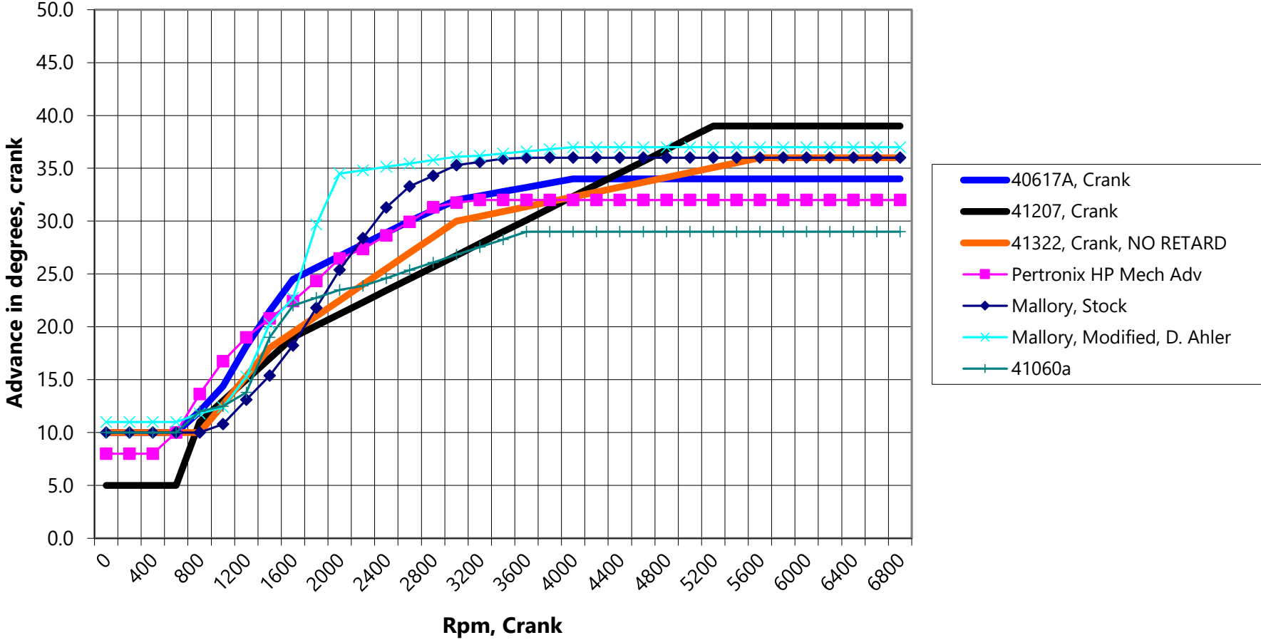
Ignition advance Curves XKE (1.3) 1-3-2012
