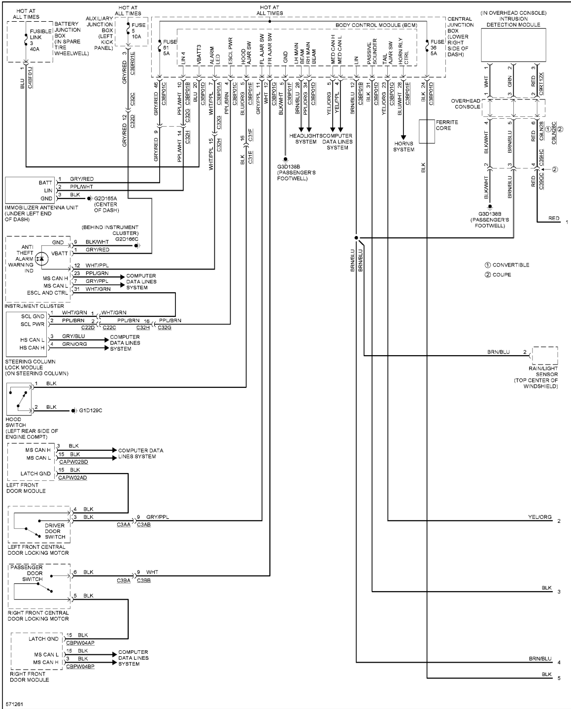
Fig. 6: Anti-theft Circuit (1 of 2)
