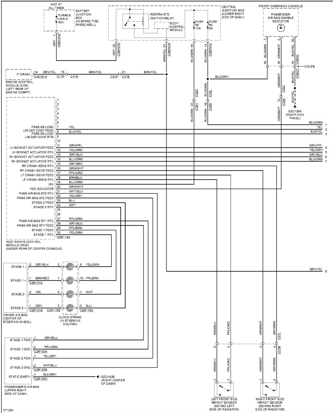
Fig. 127: Supplemental Restraints Circuit (1 of 4)
