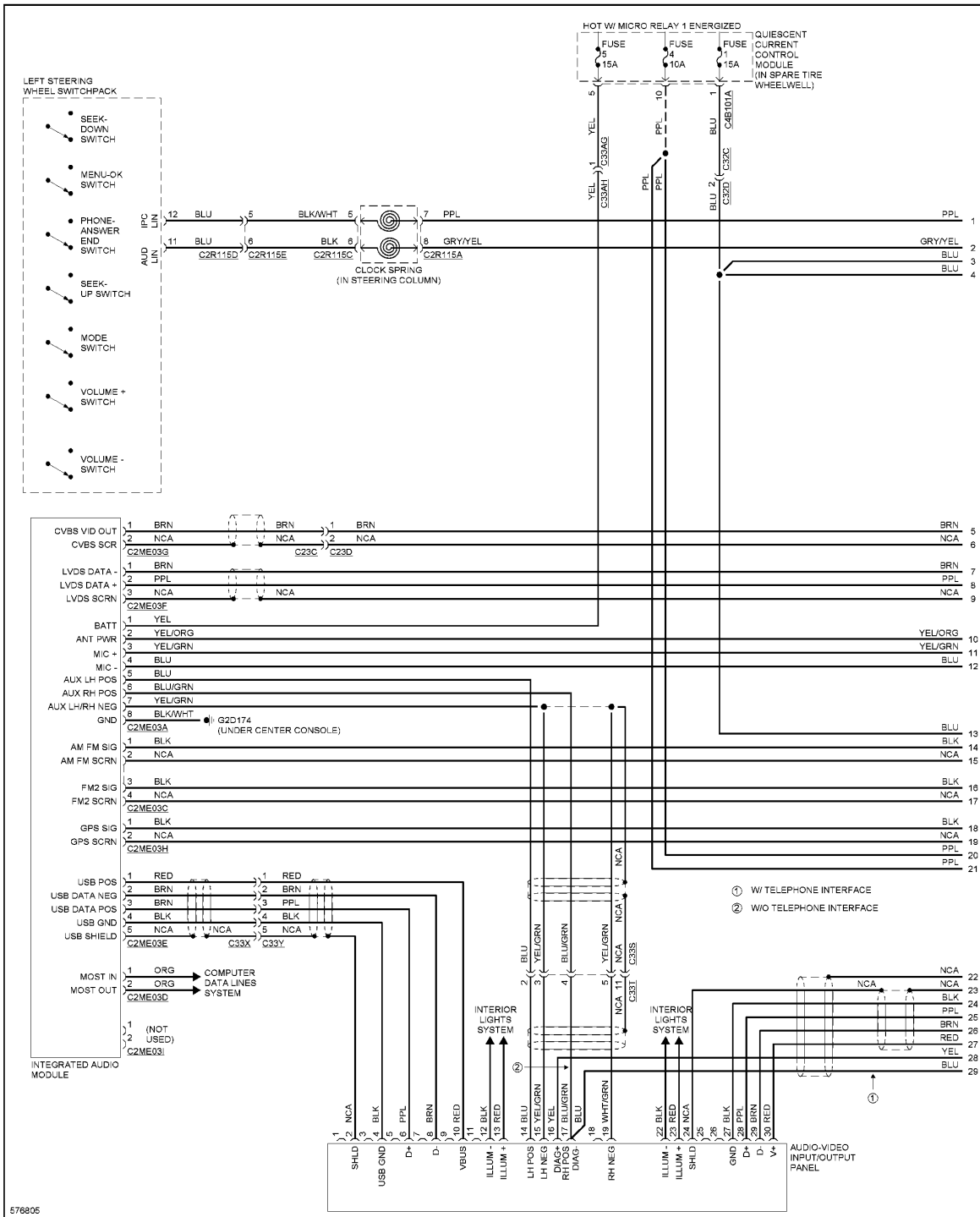
Fig. 116: Premium Radio Circuit, W/O Control Touch (1 of 6)
