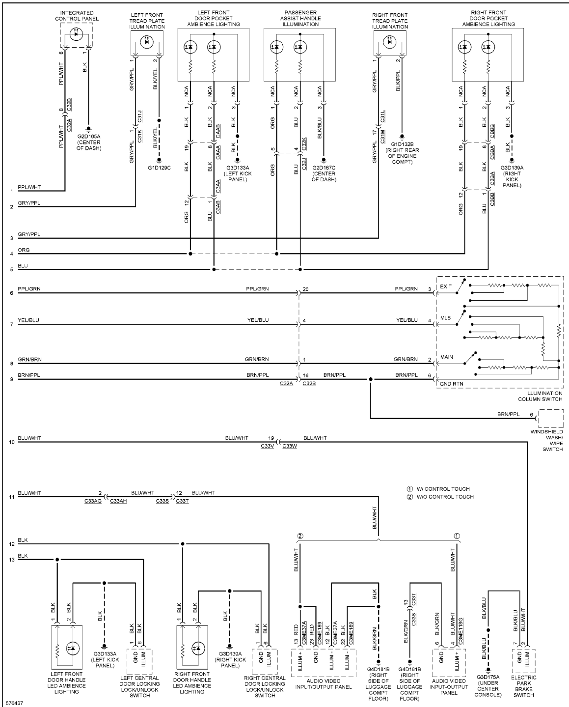
Fig. 58: Instrument Illumination Circuit (2 of 2)
