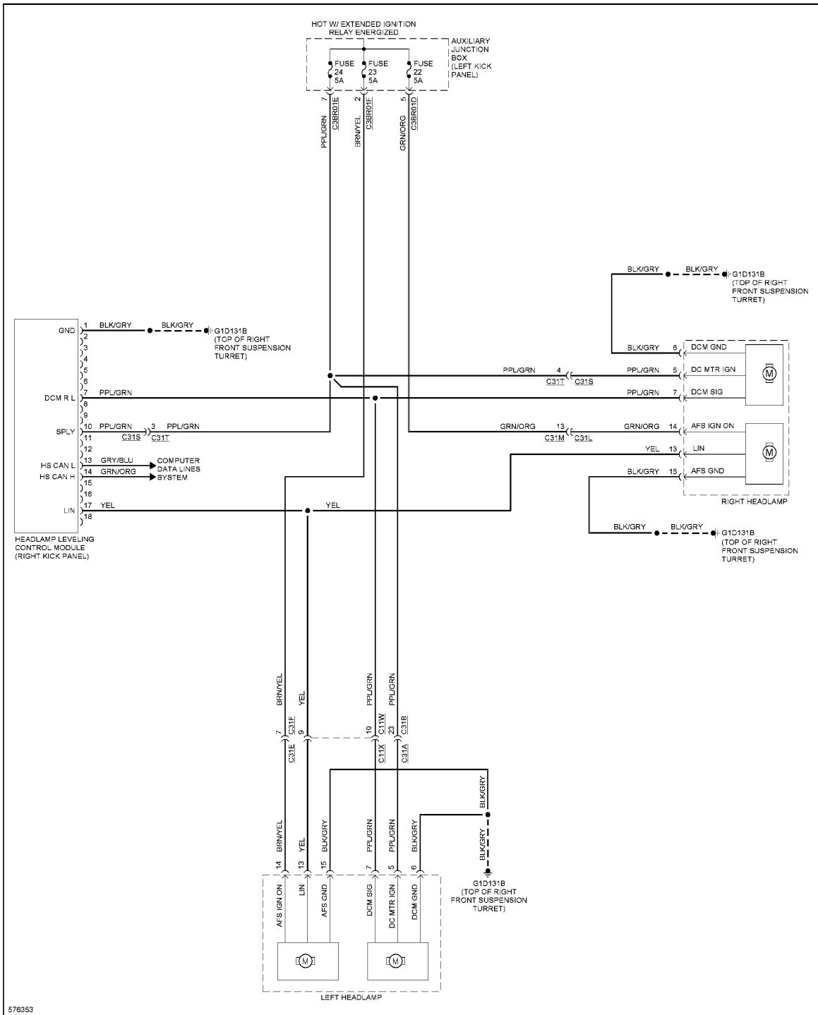
Fig. 50: Adaptive Front Lighting Circuit
