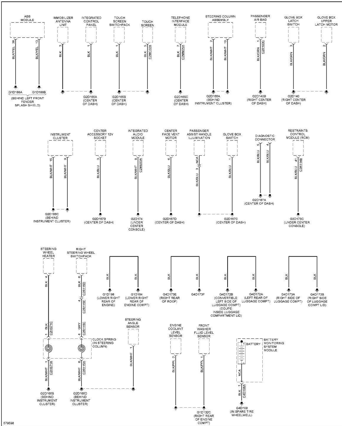
Fig. 45: Ground Distribution Circuit (2 of 6)
