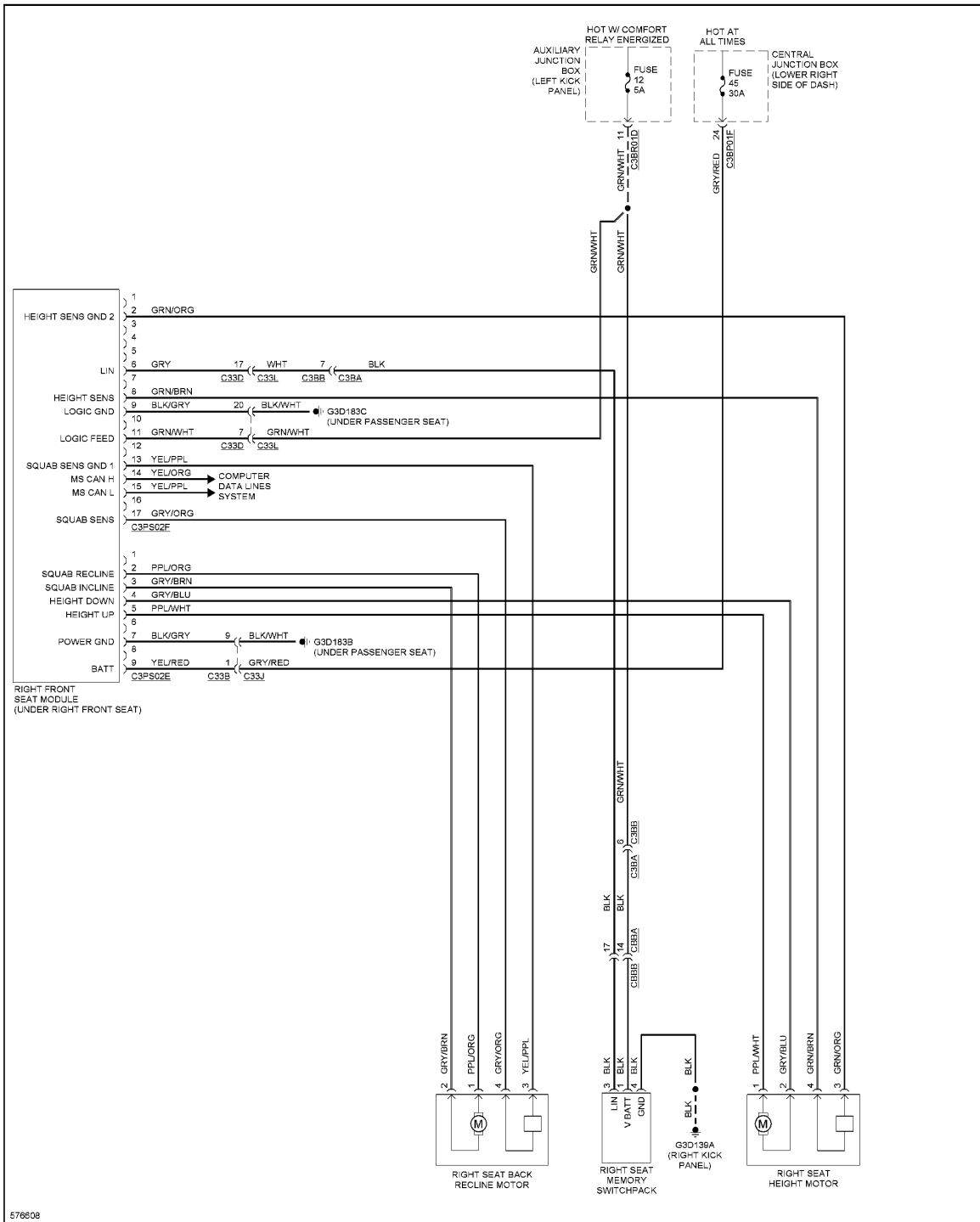
Fig. 63: Passenger's Memory Seat Circuit, 4-Way
