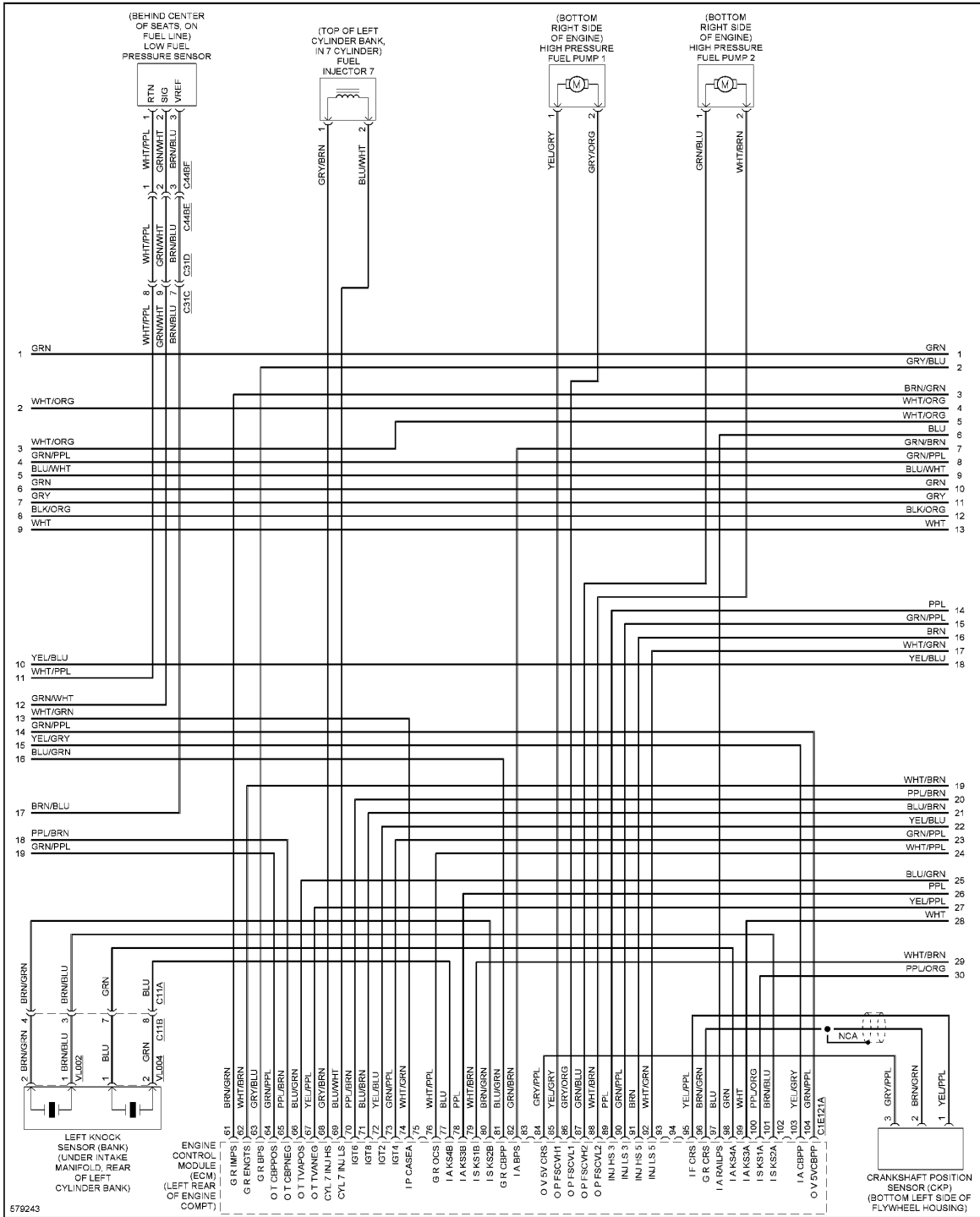
Fig. 37: 5.0L SC, Engine Performance Circuit (6 of 9)
