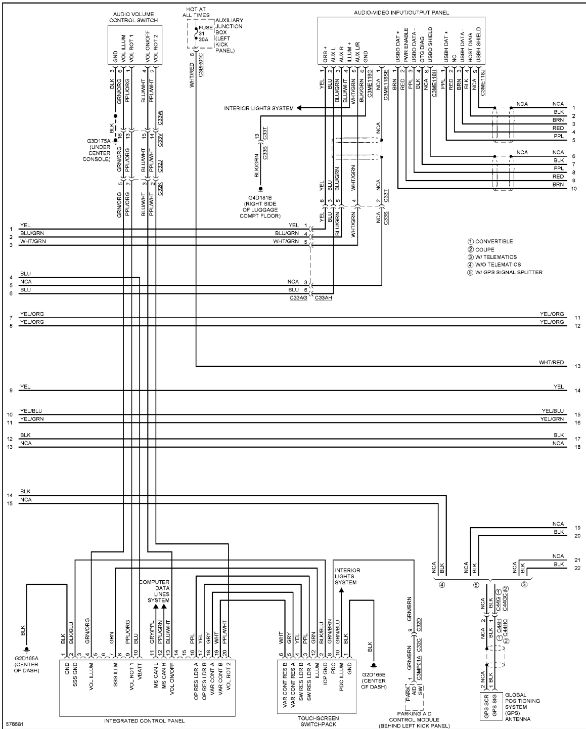
Fig. 69: Navigation Circuit, W/ Control Touch & Hi-line Audio (2 of 5)
