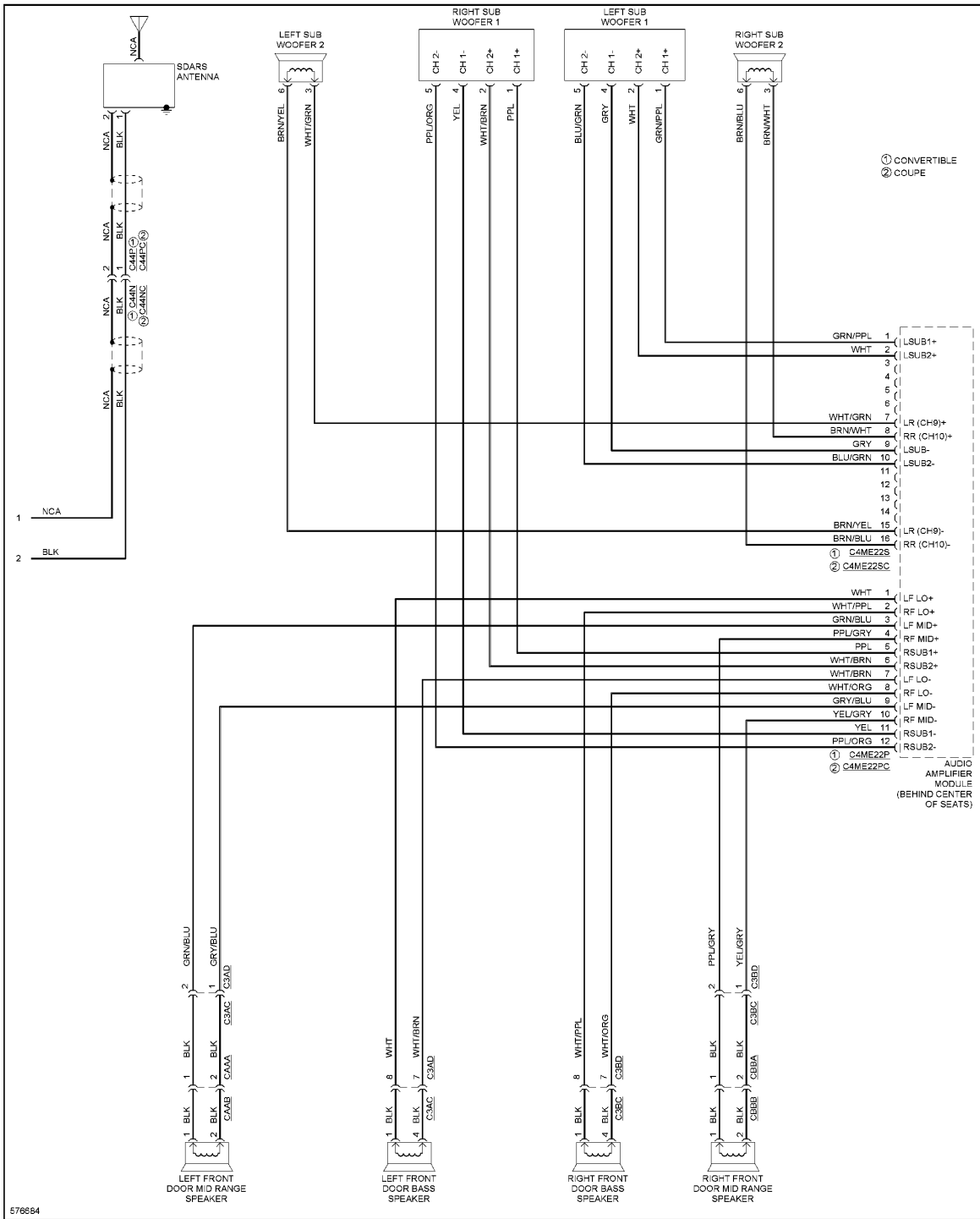
Fig. 72: Navigation Circuit, W/ Control Touch & Hi-line Audio (5 of 5)
