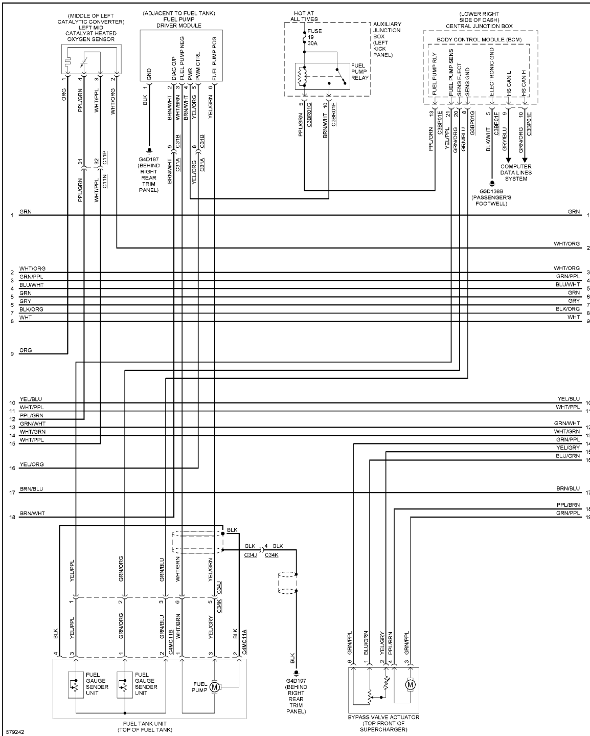
Fig. 36: 5.0L SC, Engine Performance Circuit (5 of 9)
