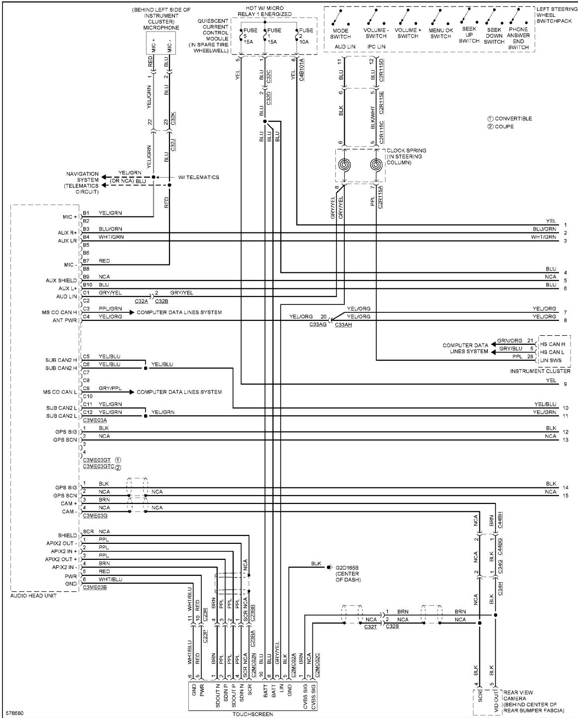
Fig. 68: Navigation Circuit, W/ Control Touch & Hi-line Audio (1 of 5)
