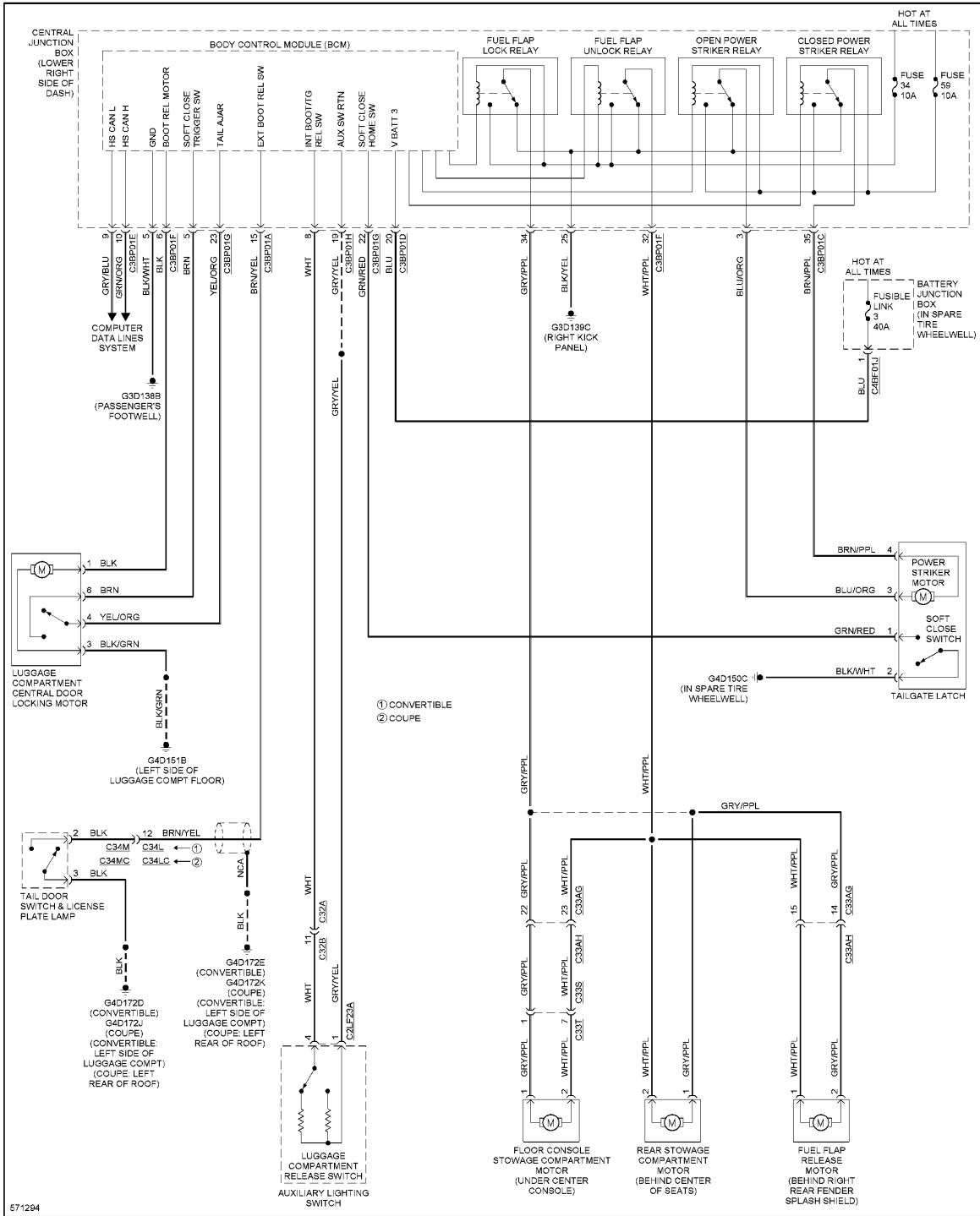
Fig. 135: Tailgate & Fuel Door Release Circuit
