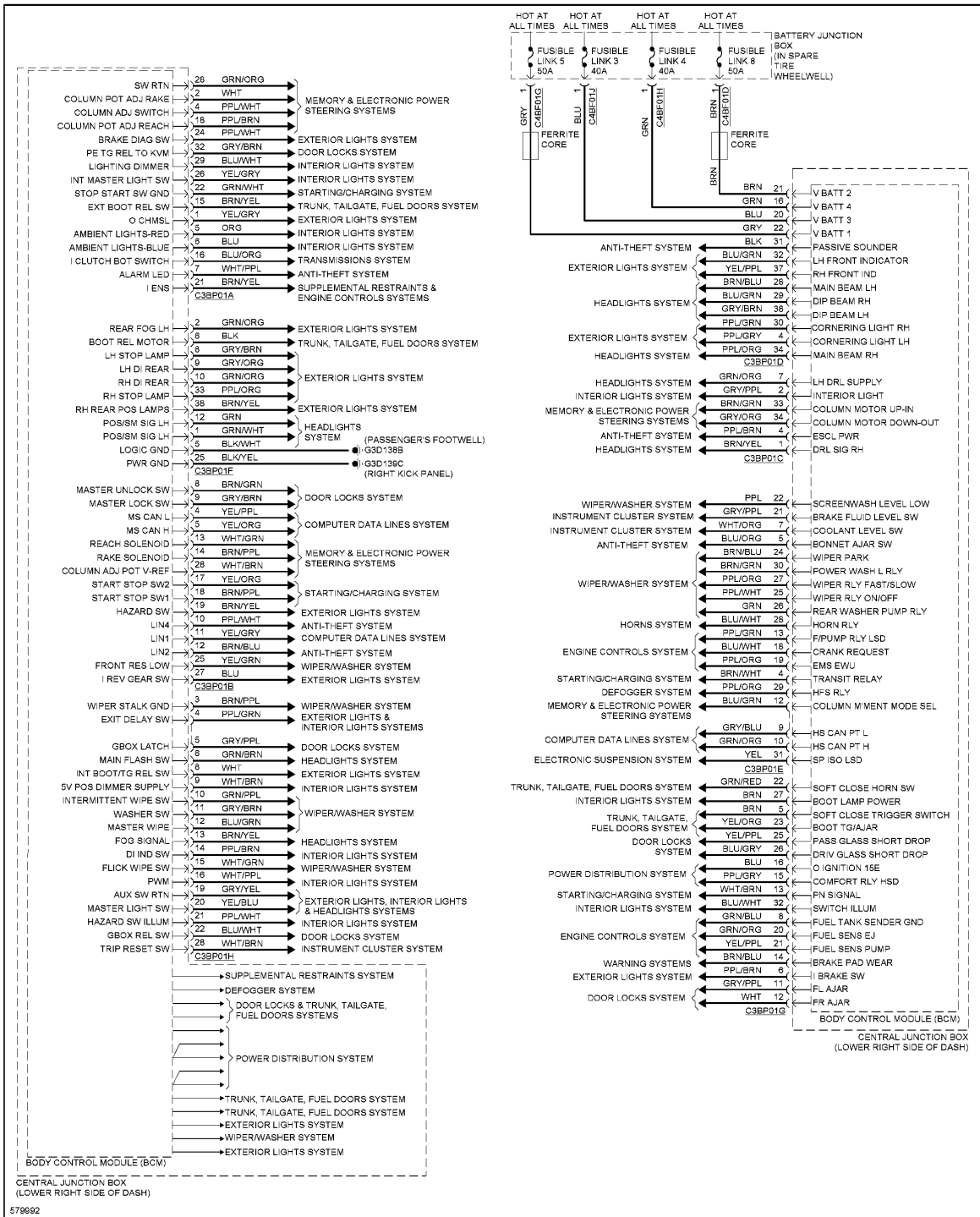
Fig. 8: Body Control Modules Circuit
