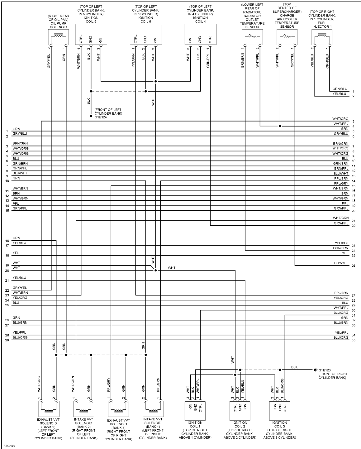
Fig. 30: 3.0L SC, Engine Performance Circuit (8 of 9)
