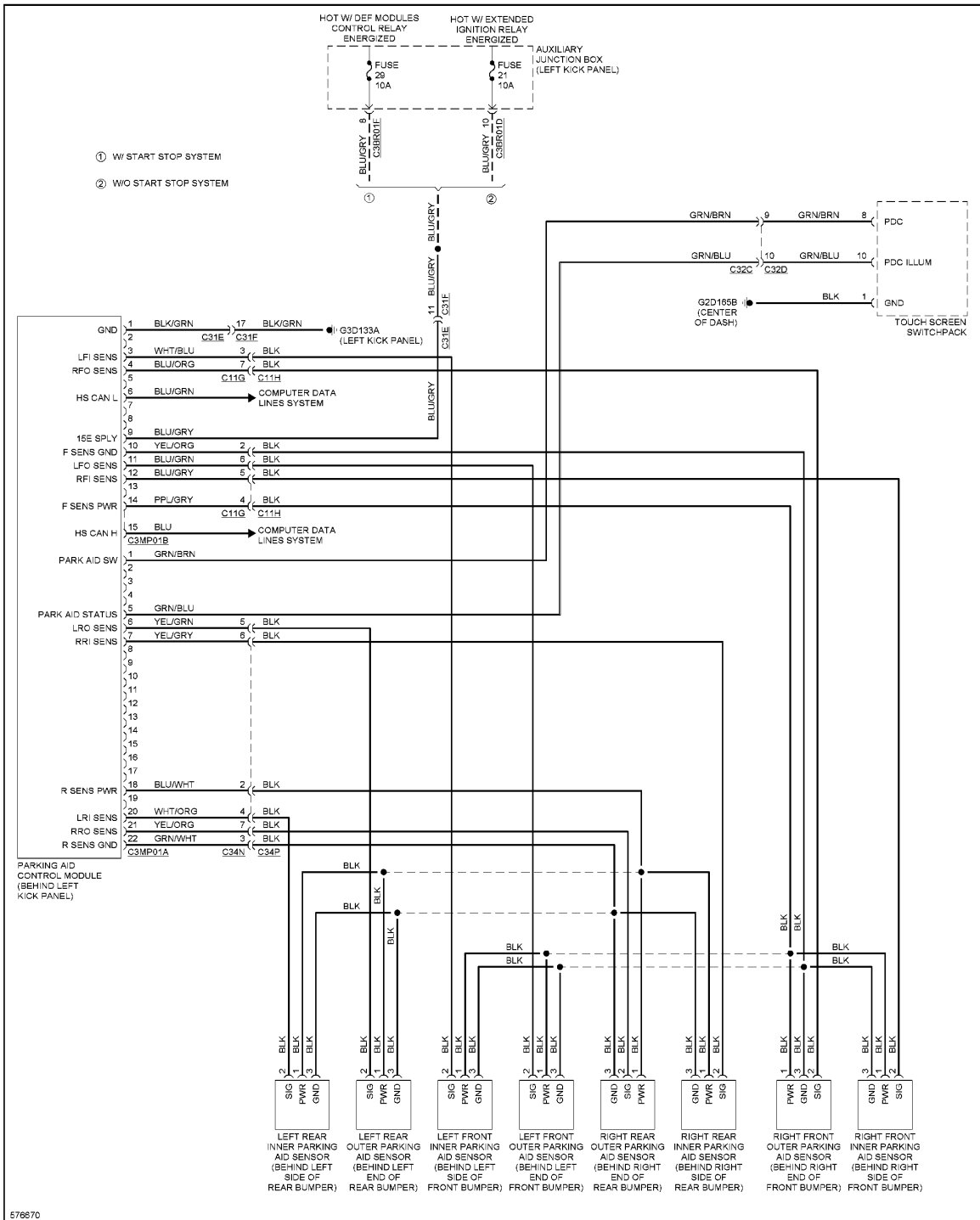
Fig. 84: Parking Assistant Circuit
