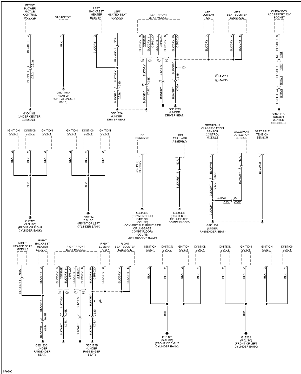
Fig. 47: Ground Distribution Circuit (4 of 6)
