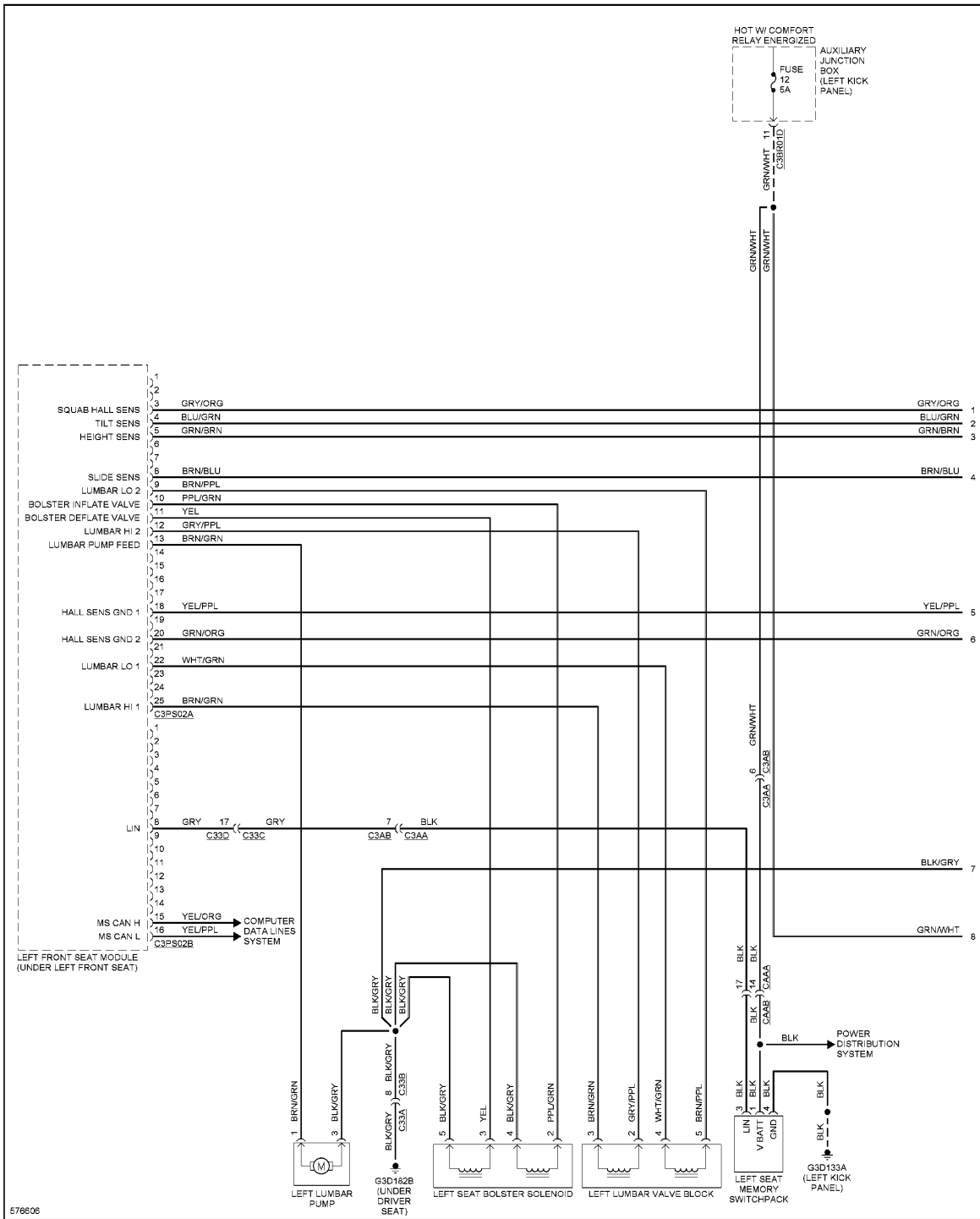
Fig. 60: Driver's Memory Seat Circuit, 8-Way (1 of 2)
