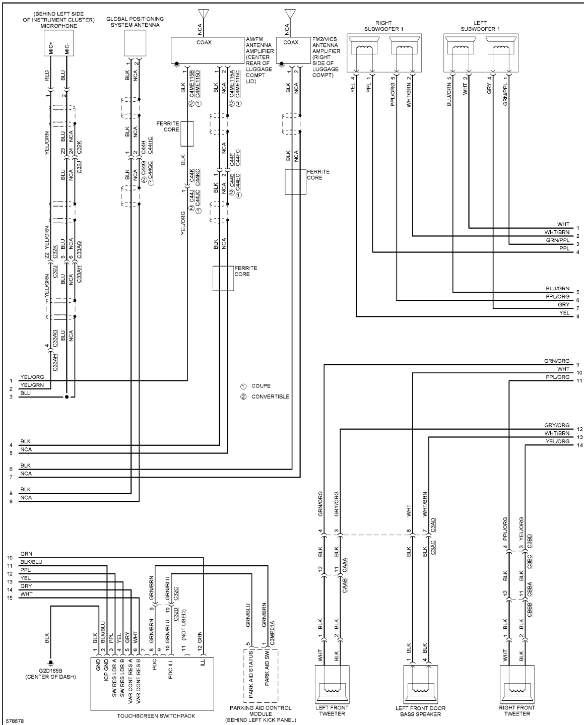
Fig. 82: Navigation Circuit, W/O Control Touch (5 of 6)
