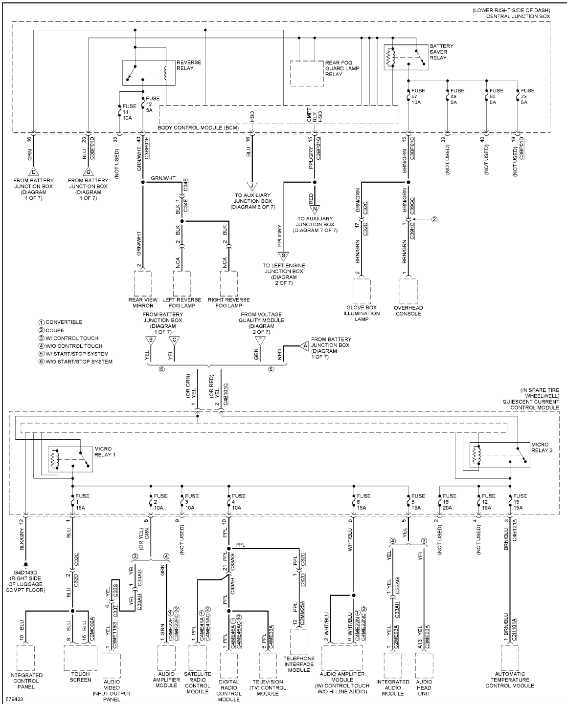
Fig. 92: Power Distribution Circuit (5 of 7)
