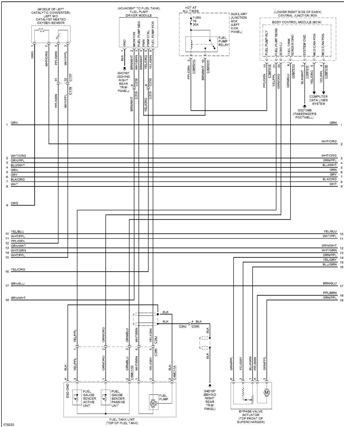
Fig. 27: 3.0L SC, Engine Performance Circuit (5 of 9)
