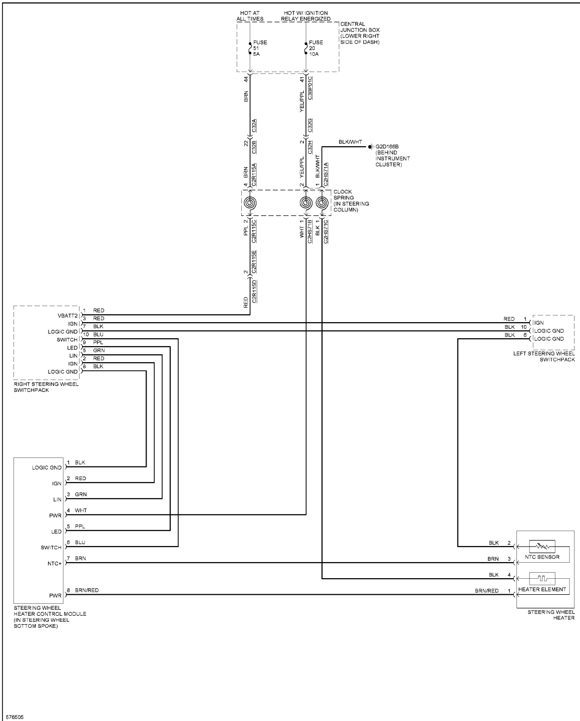
Fig. 102: Heated Steering Wheel Circuit
