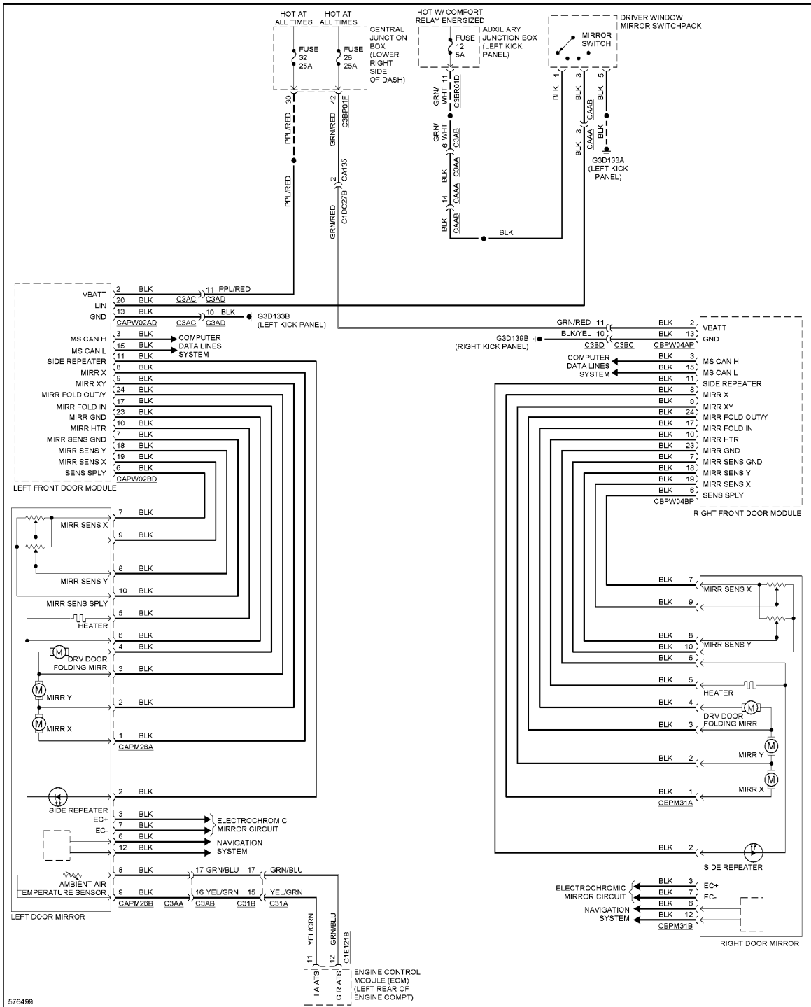
Fig. 100: Power Mirrors Circuit
