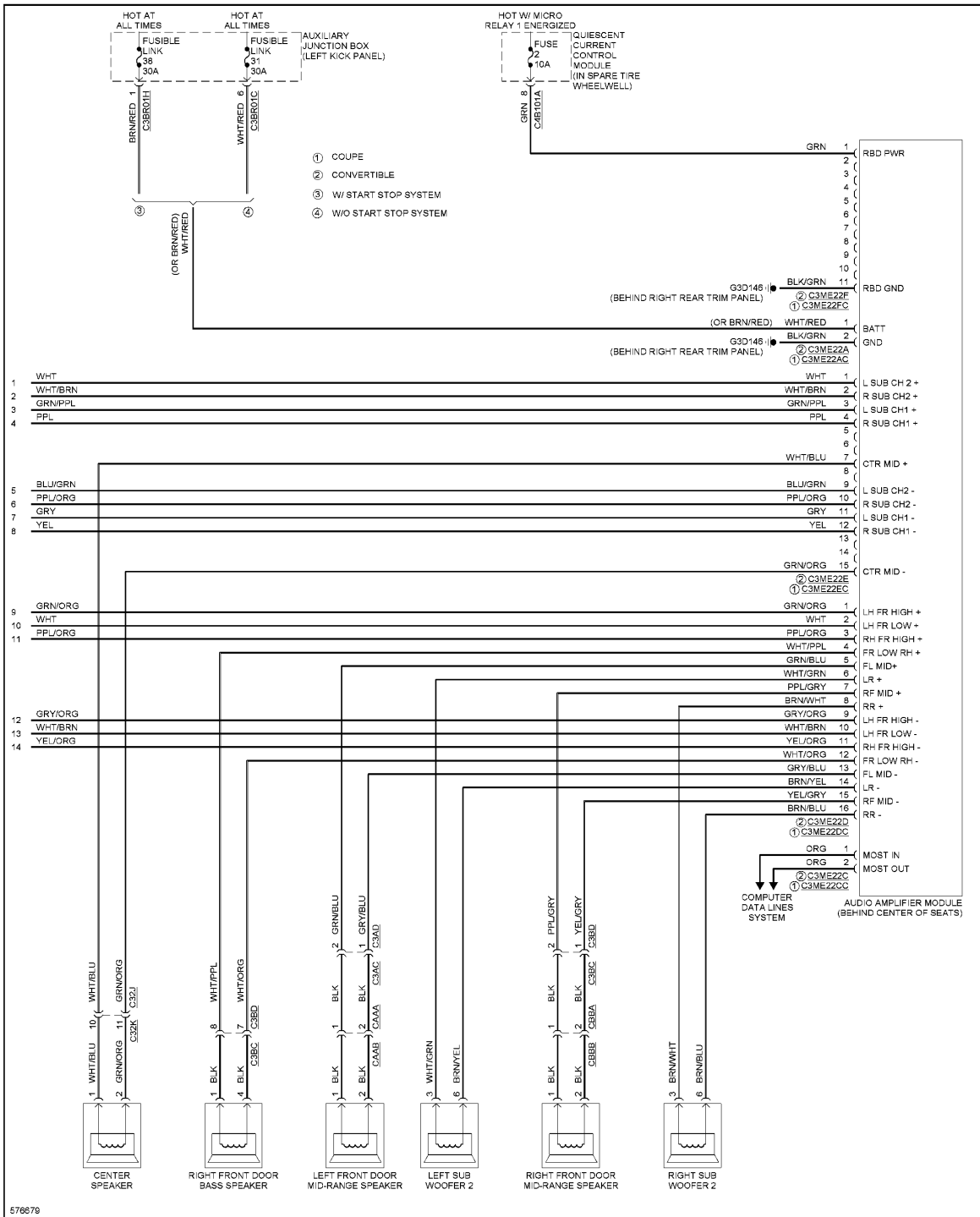
Fig. 83: Navigation Circuit, W/O Control Touch (6 of 6)
