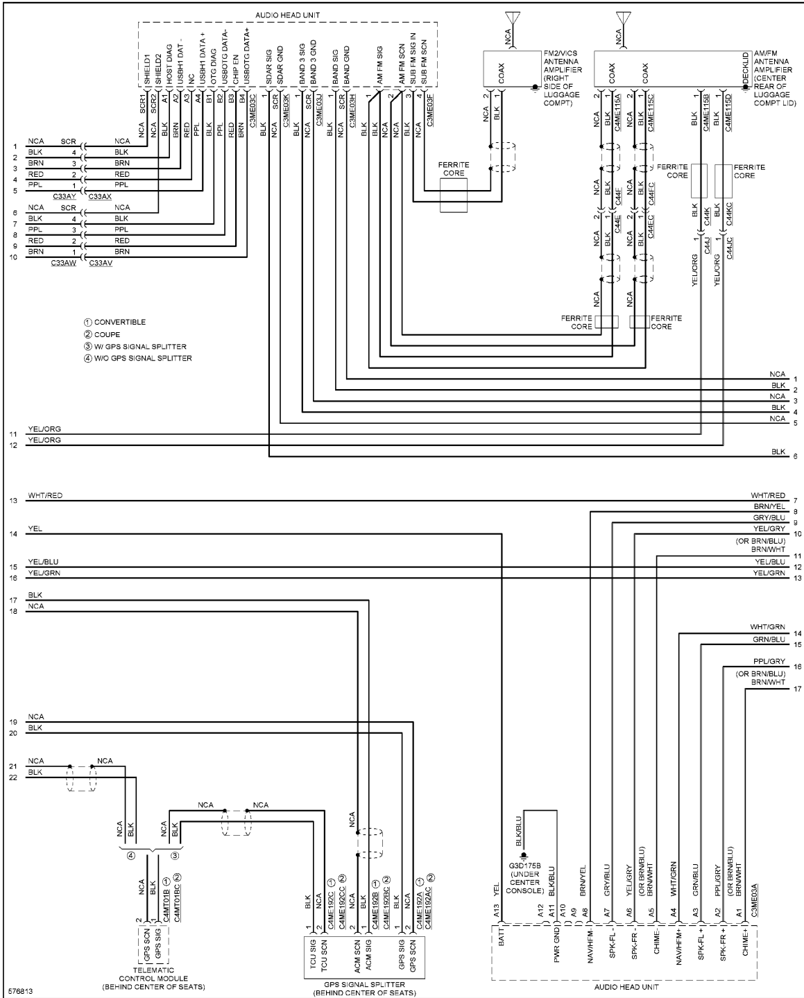
Fig. 108: Premium Radio Circuit, W/ Control Touch & Hi-line Audio (3 of 5)
