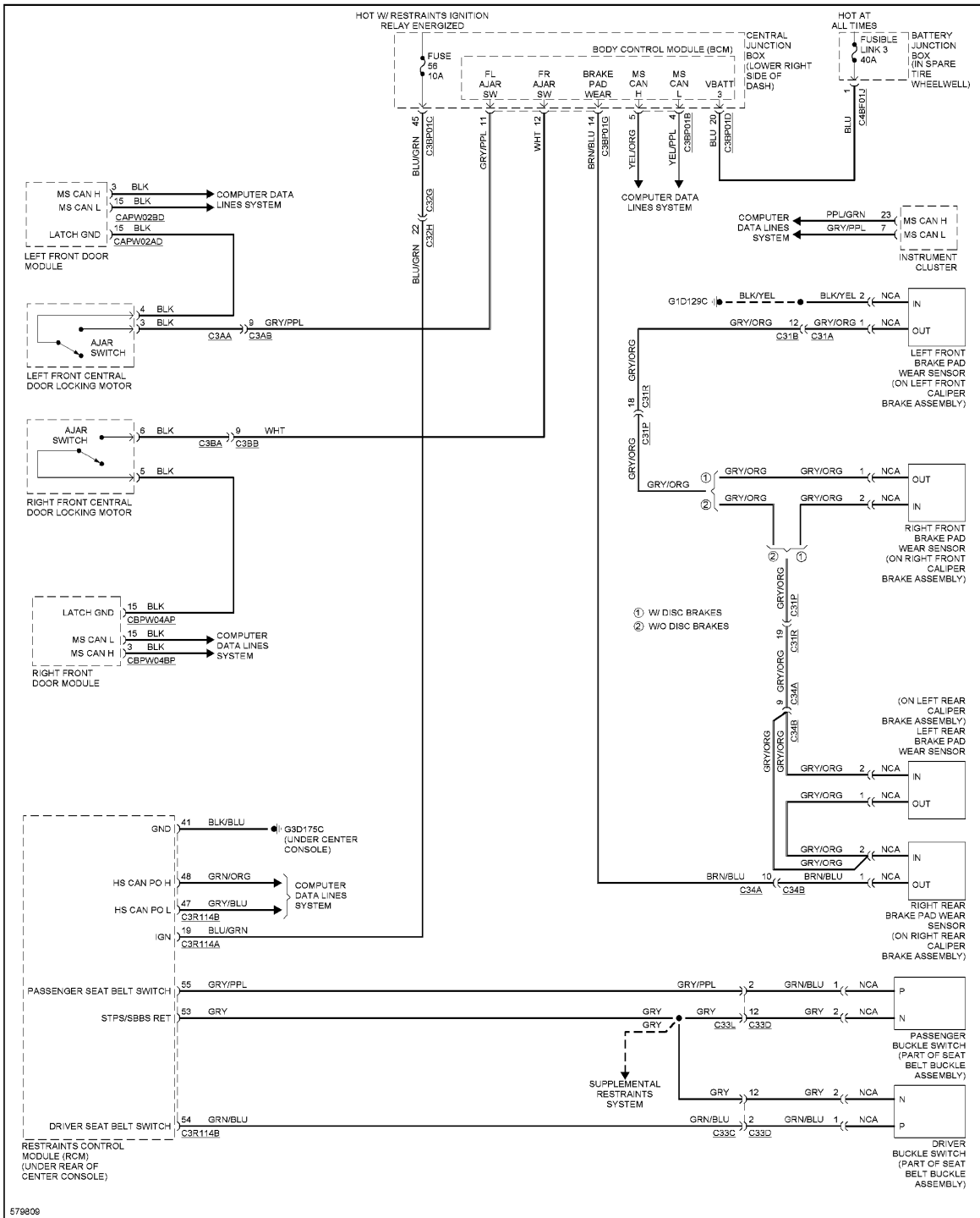
Fig. 136: Seat Belt Warning Circuit
