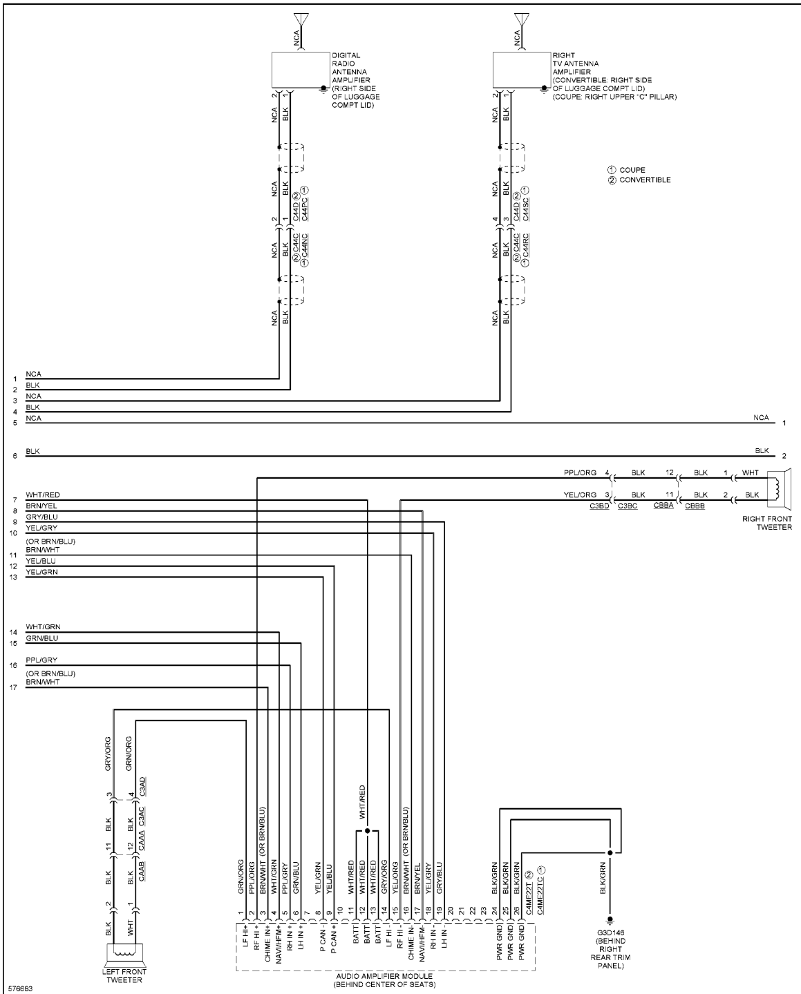
Fig. 71: Navigation Circuit, W/ Control Touch & Hi-line Audio (4 of 5)
