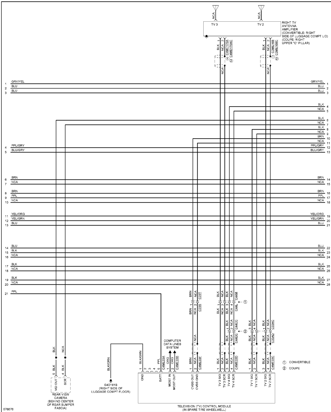
Fig. 80: Navigation Circuit, W/O Control Touch (3 of 6)
