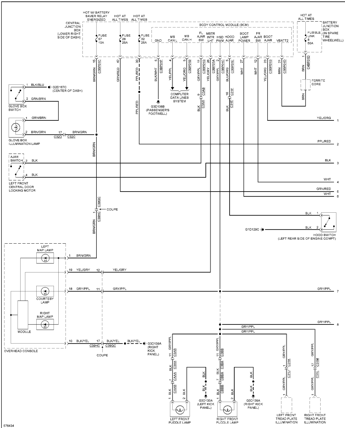
Fig. 55: Courtesy Lamps Circuit (1 of 2)
