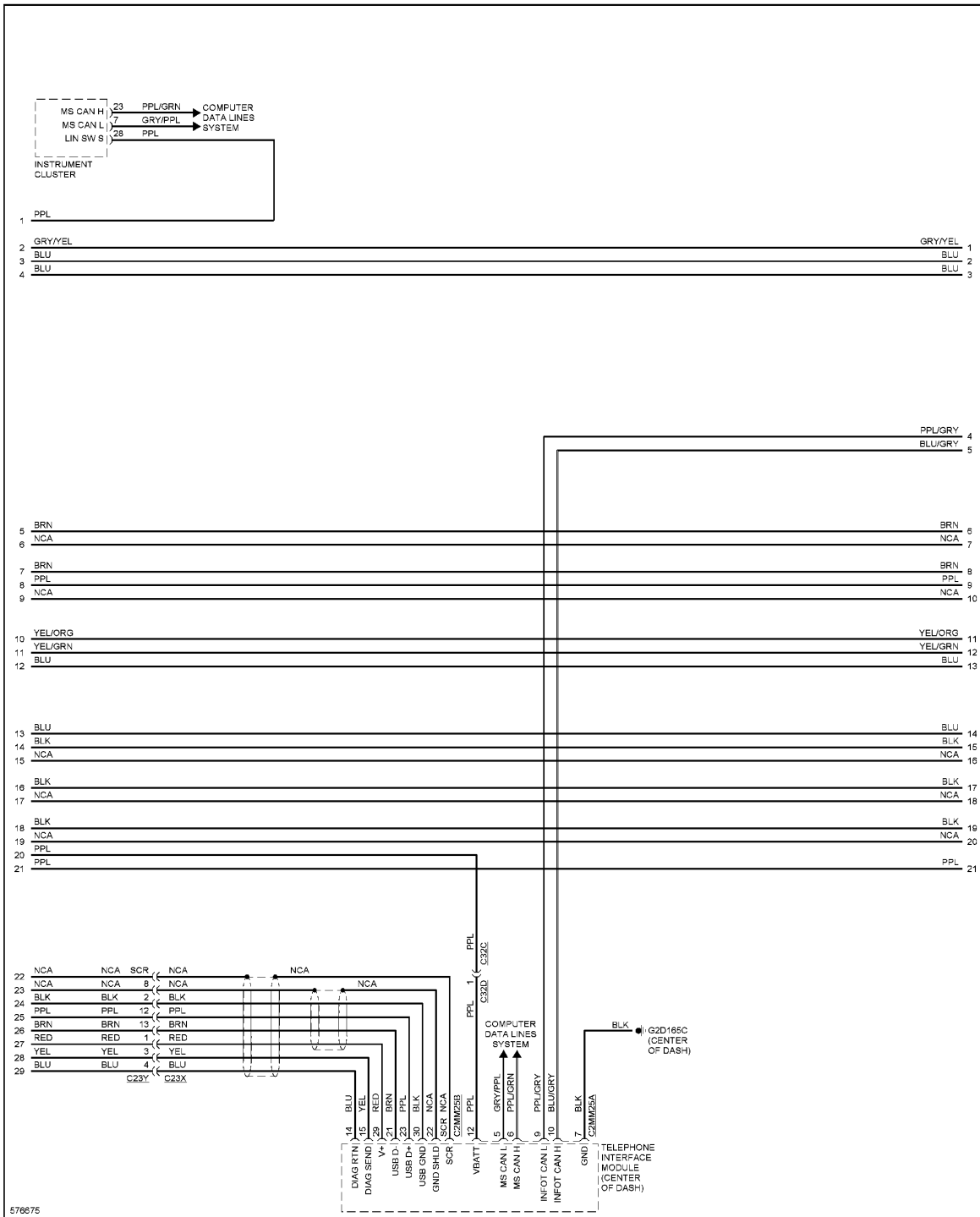
Fig. 79: Navigation Circuit, W/O Control Touch (2 of 6)
