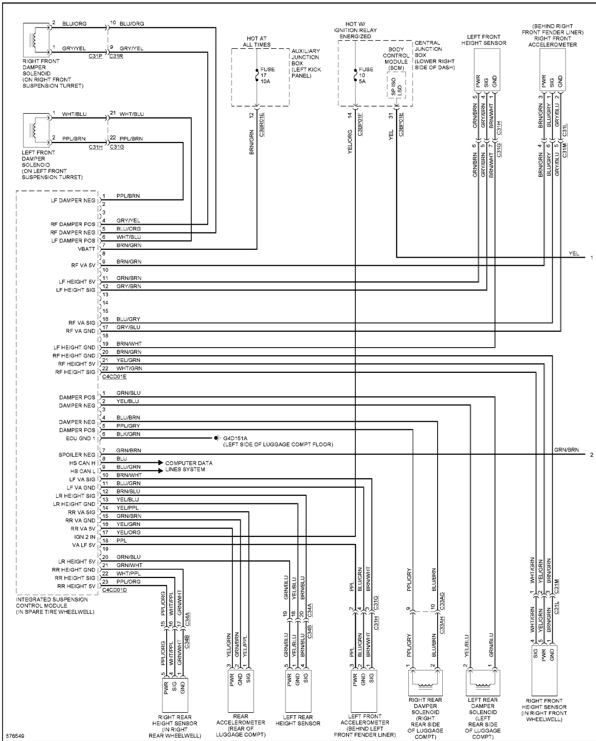
Fig. 21: Electronic Suspension Circuit (1 of 2)
