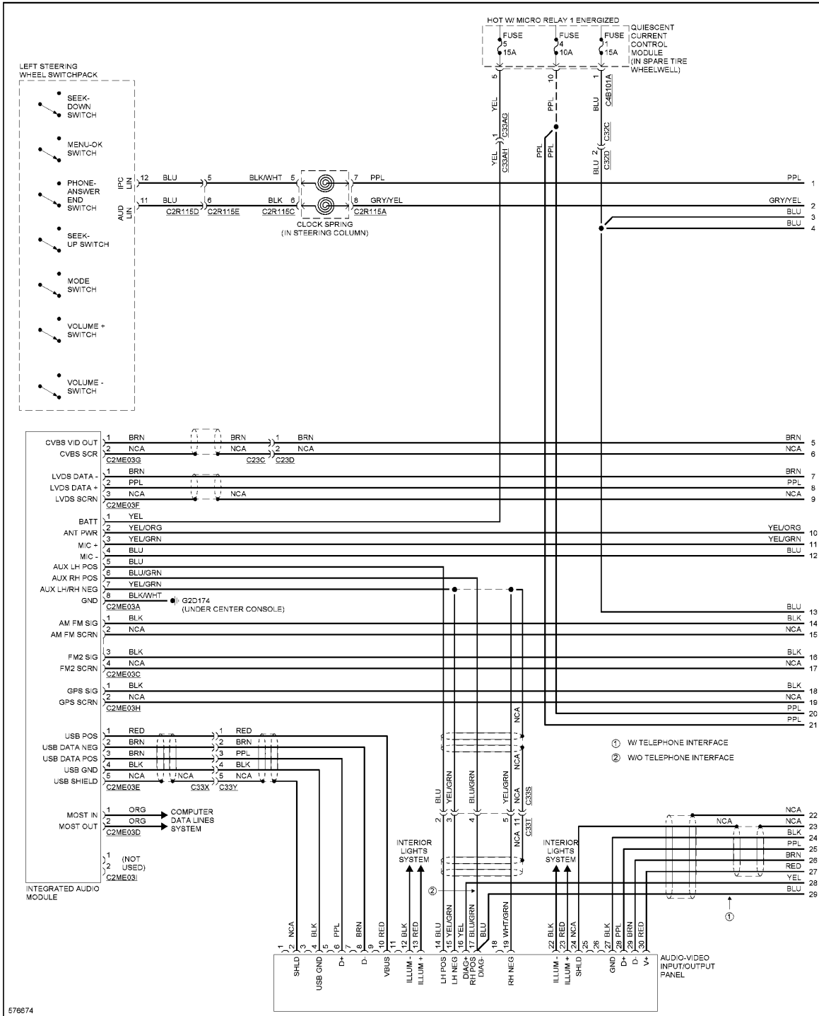
Fig. 78: Navigation Circuit, W/O Control Touch (1 of 6)
