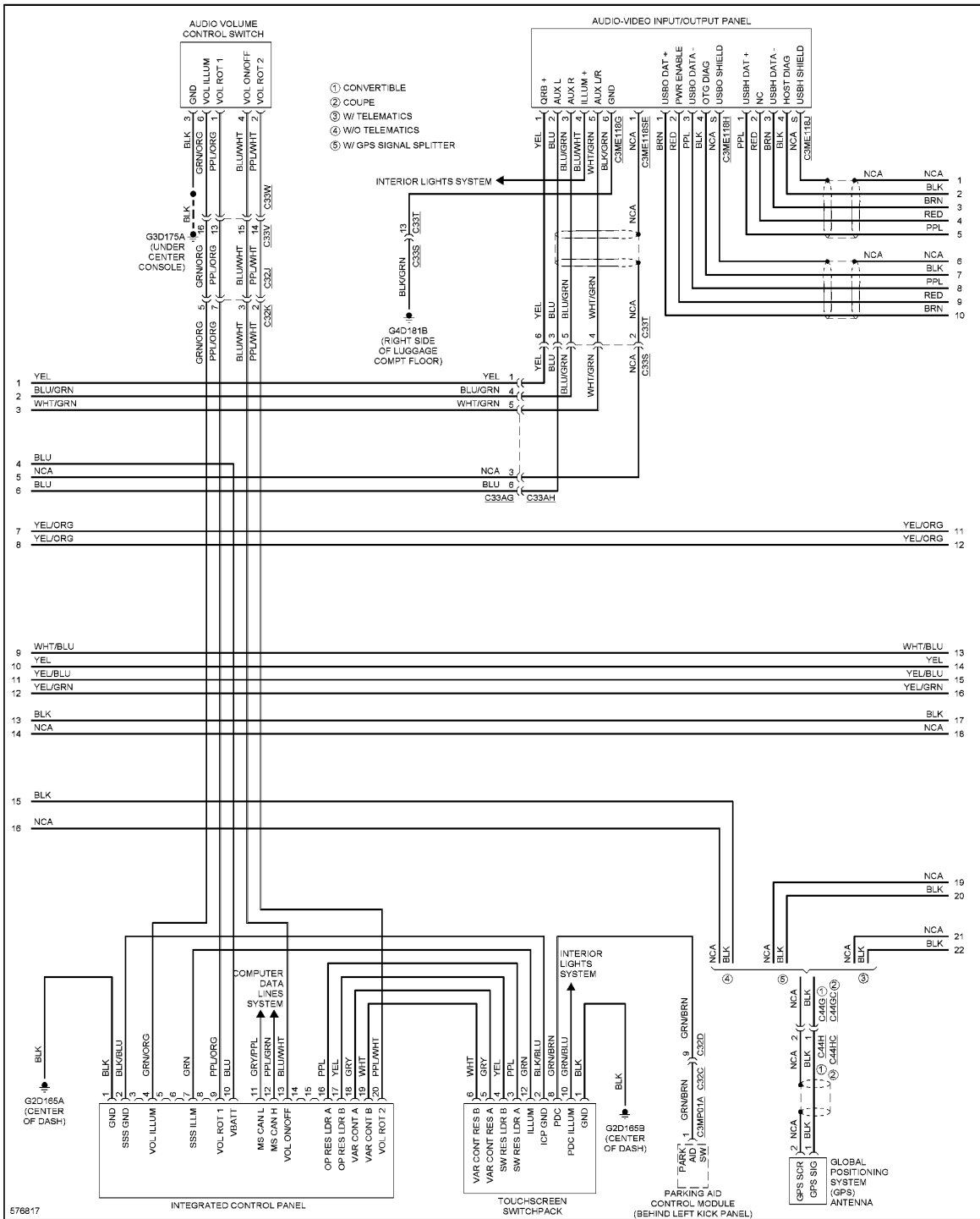
Fig. 112: Premium Radio Circuit, W/ Control Touch W/O Hi-line Audio (2 of 5)
