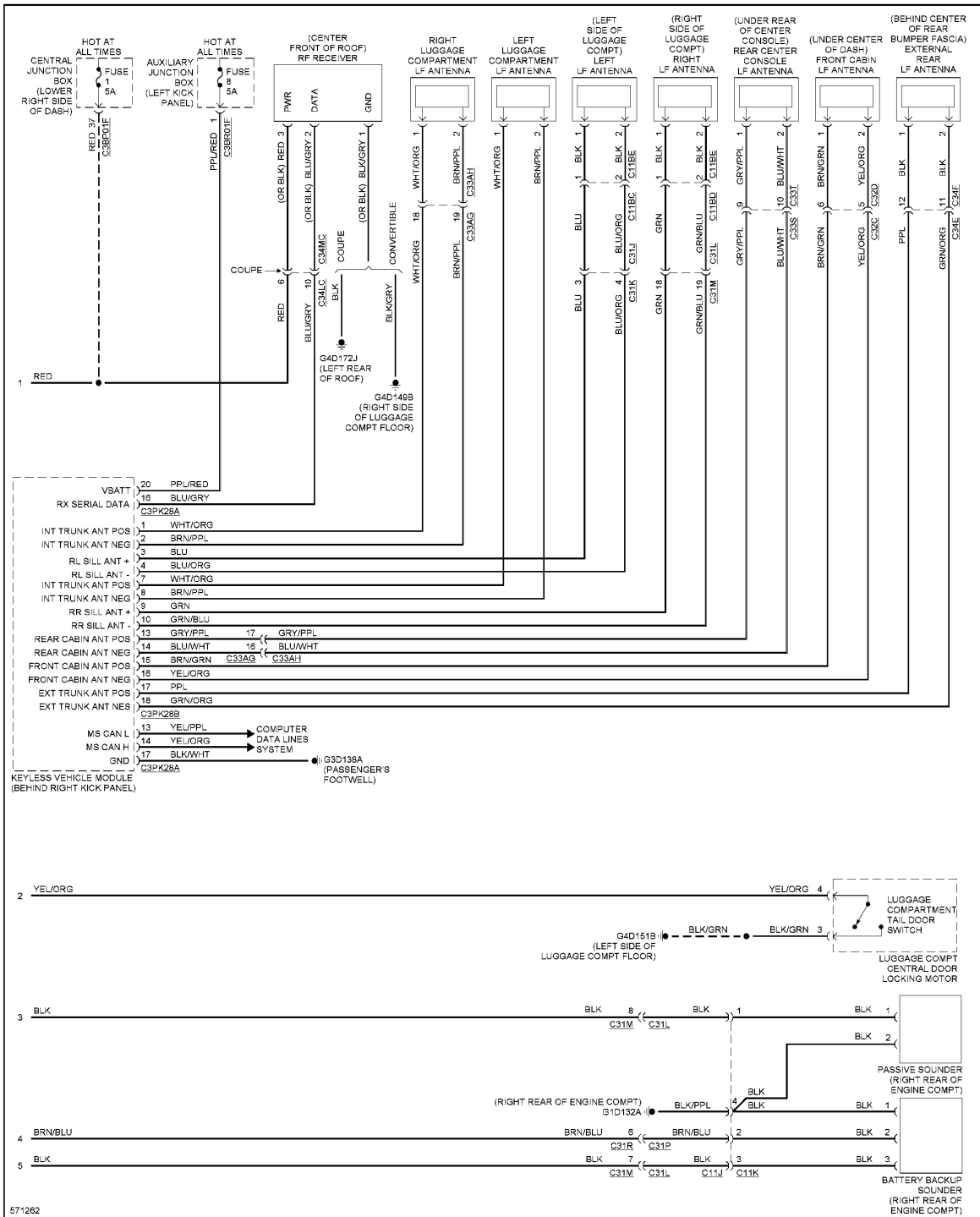
Fig. 7: Anti-theft Circuit (2 of 2)
