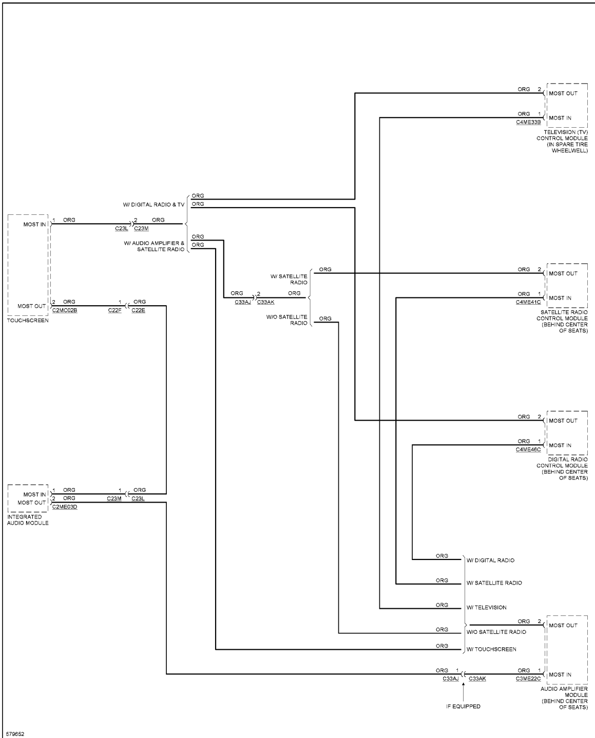
Fig. 13: Fibre Optic Network Circuit, Convertible
