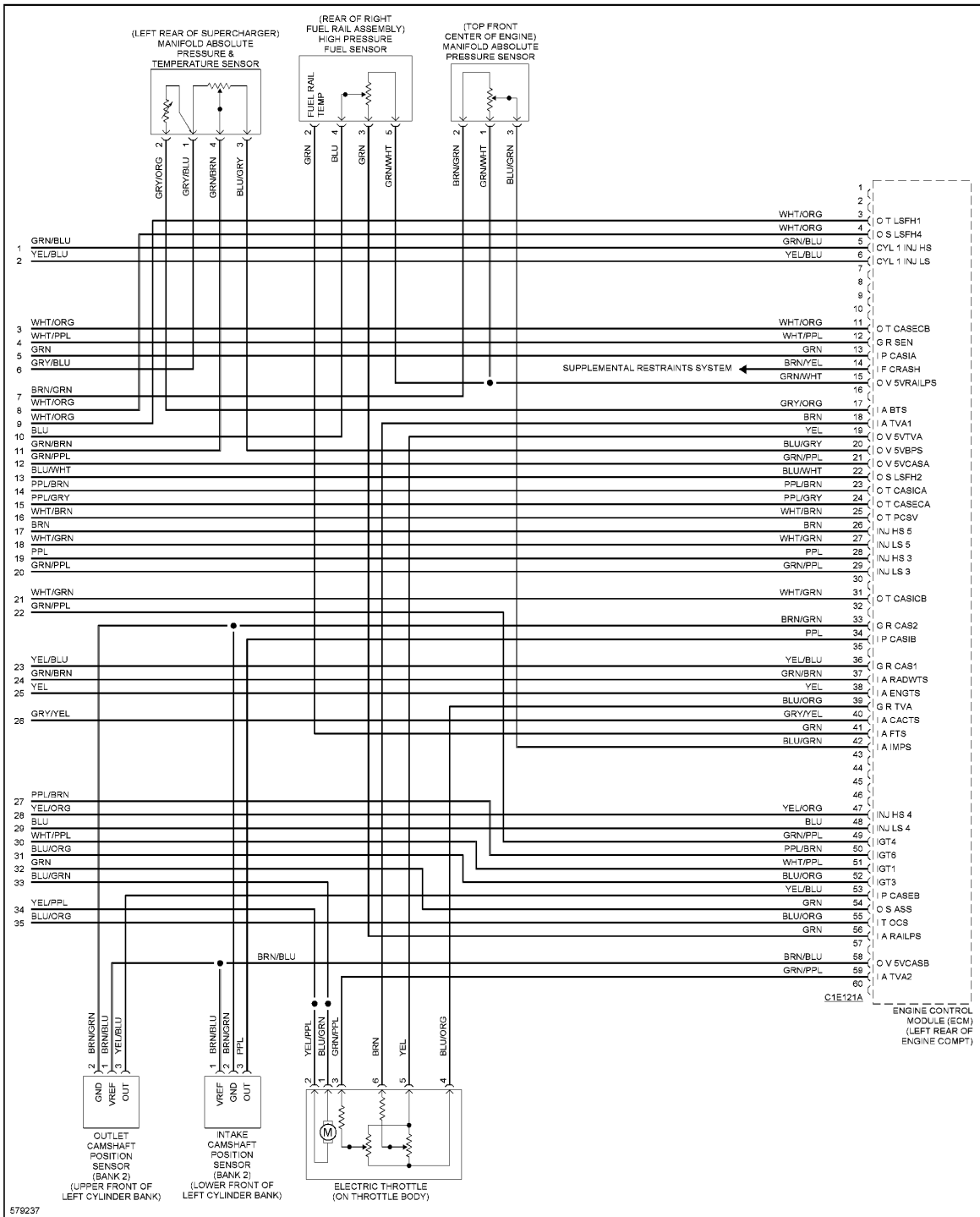
Fig. 31: 3.0L SC, Engine Performance Circuit (9 of 9)
