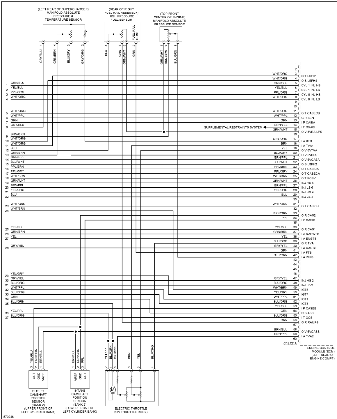
Fig. 40: 5.0L SC, Engine Performance Circuit (9 of 9)
