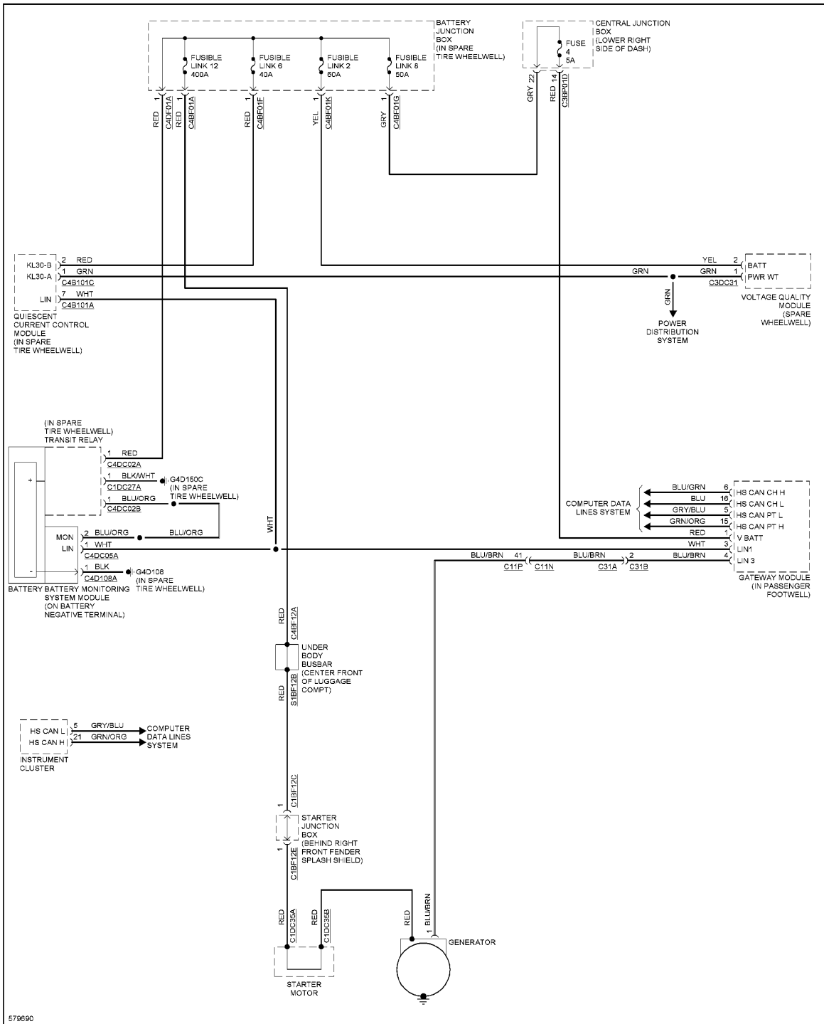
Fig. 124: Charging Circuit, W/ Start-Stop System
