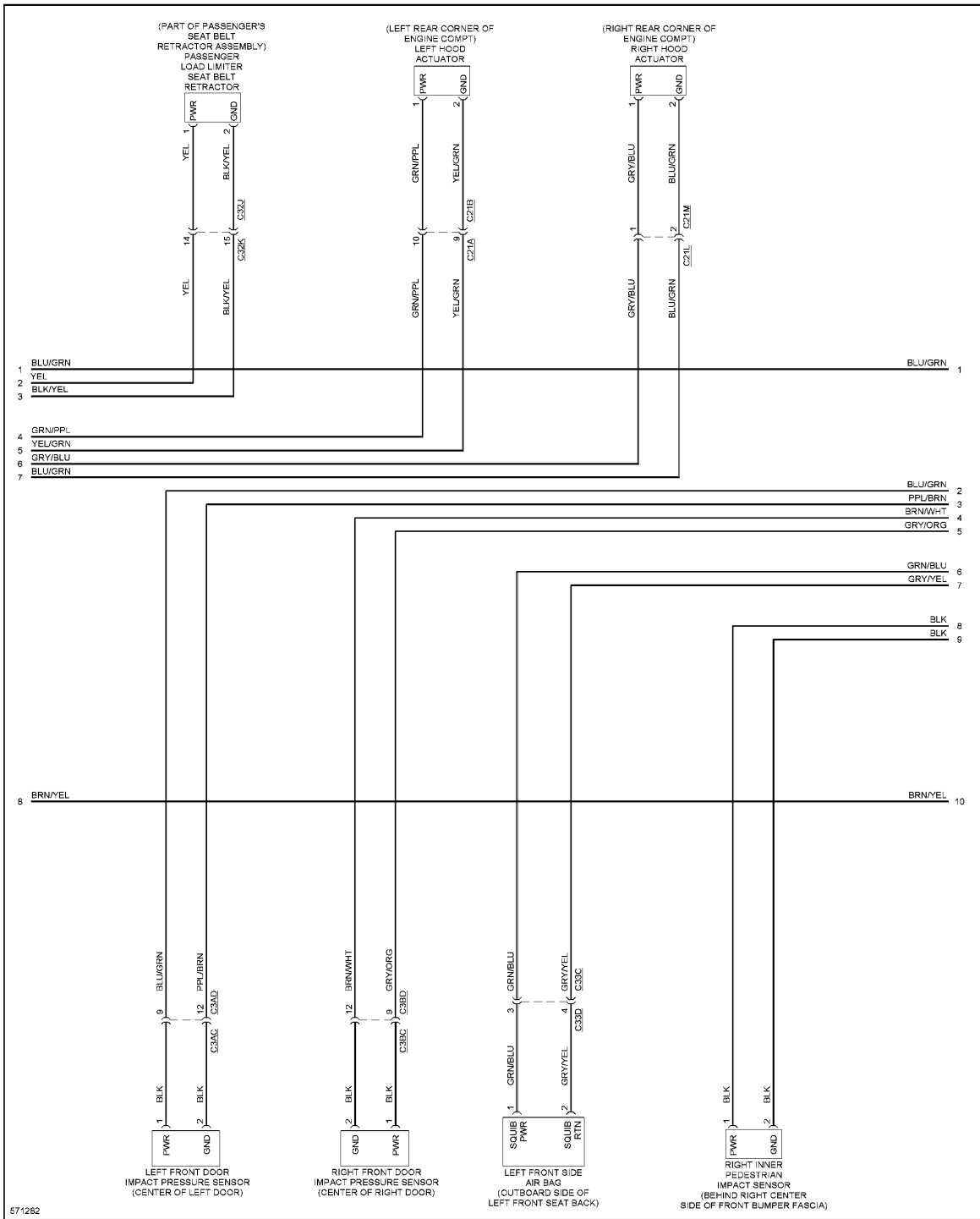
Fig. 128: Supplemental Restraints Circuit (2 of 4)
