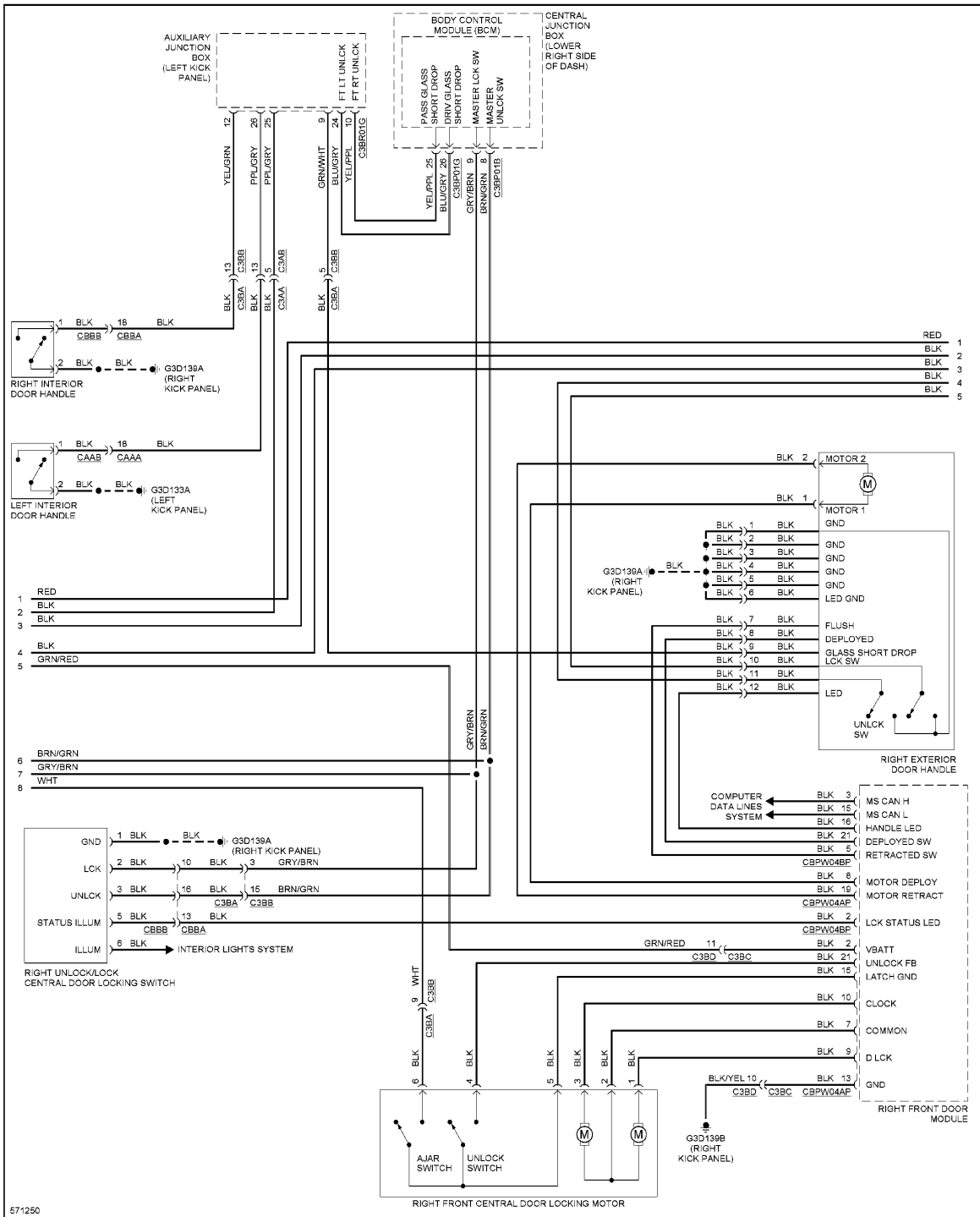
Fig. 96: Power Door Locks Circuit (2 of 4)
