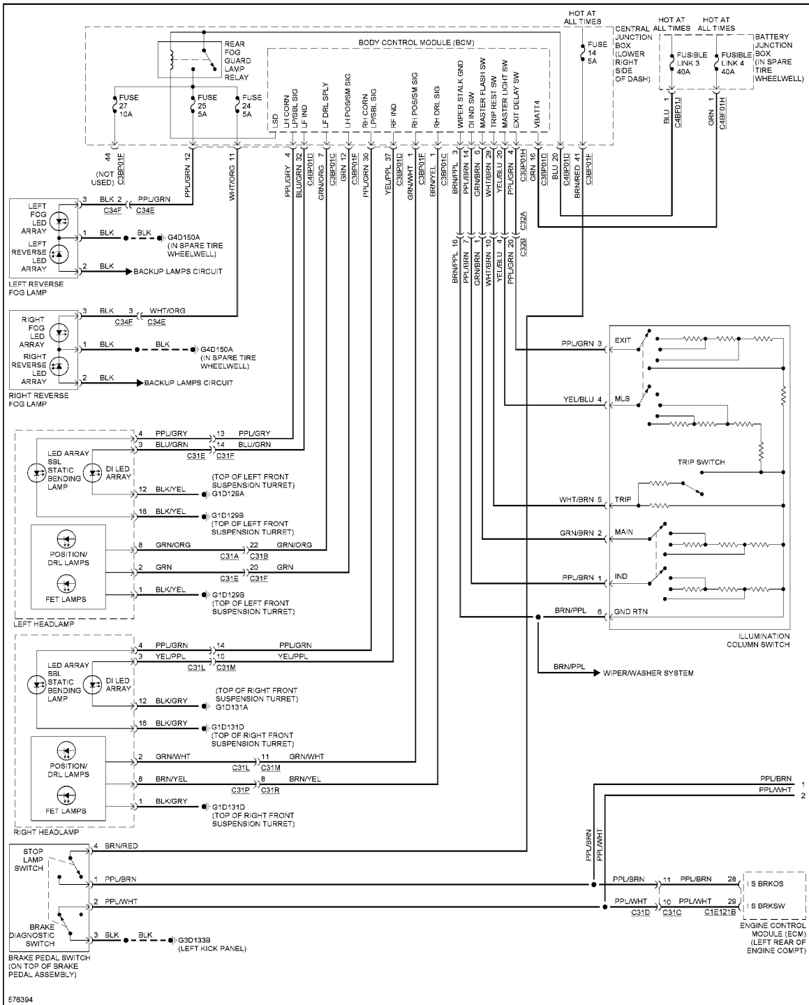
Fig. 42: Exterior Lamps Circuit (1 of 2)
