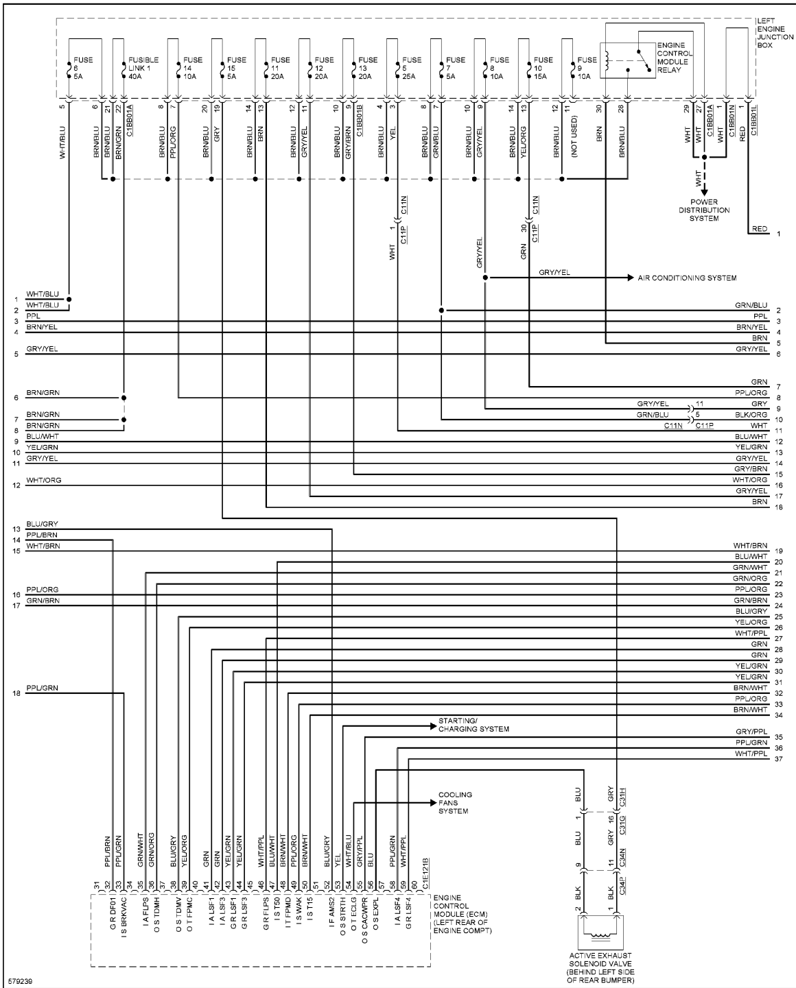
Fig. 33: 5.0L SC, Engine Performance Circuit (2 of 9)
