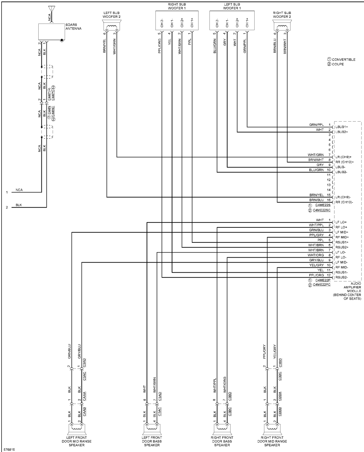
Fig. 110: Premium Radio Circuit, W/ Control Touch & Hi-line Audio (5 of 5)
