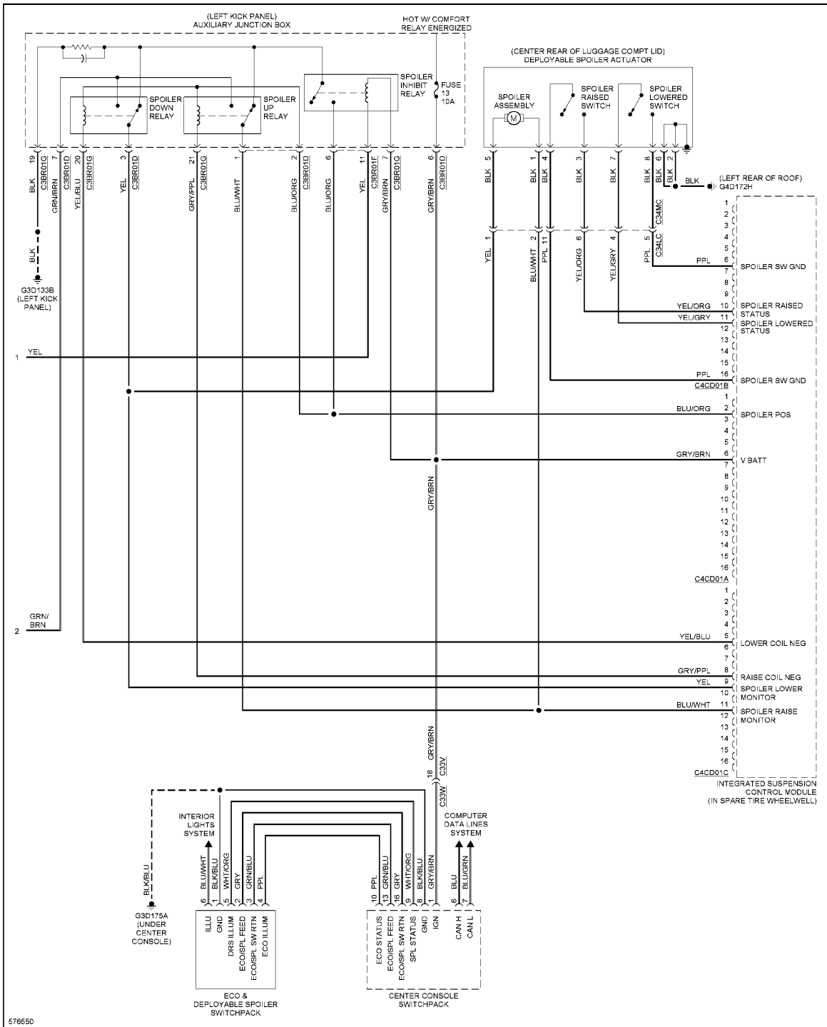
Fig. 22: Electronic Suspension Circuit (2 of 2)
