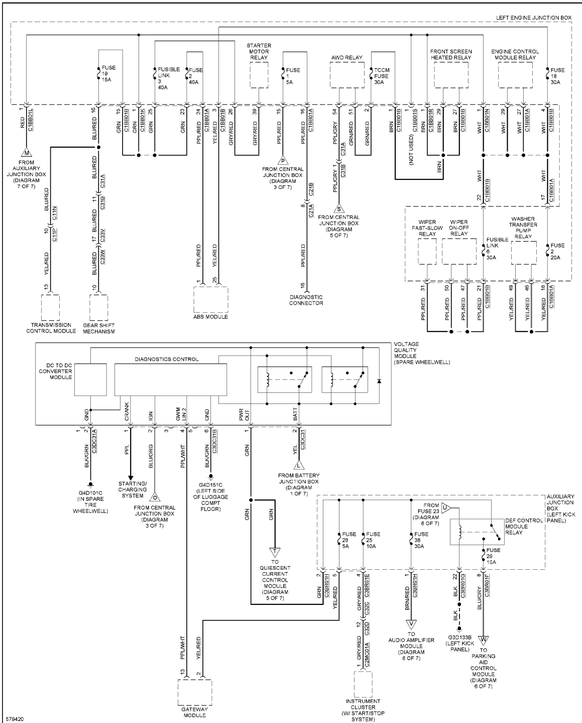
Fig. 89: Power Distribution Circuit (2 of 7)
