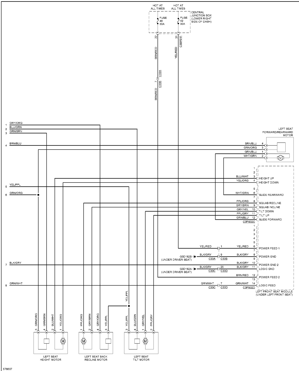
Fig. 61: Driver's Memory Seat Circuit, 8-Way (2 of 2)
