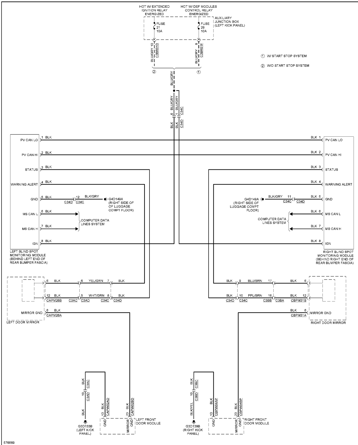
Fig. 67: Blind Spot Monitoring Circuit
