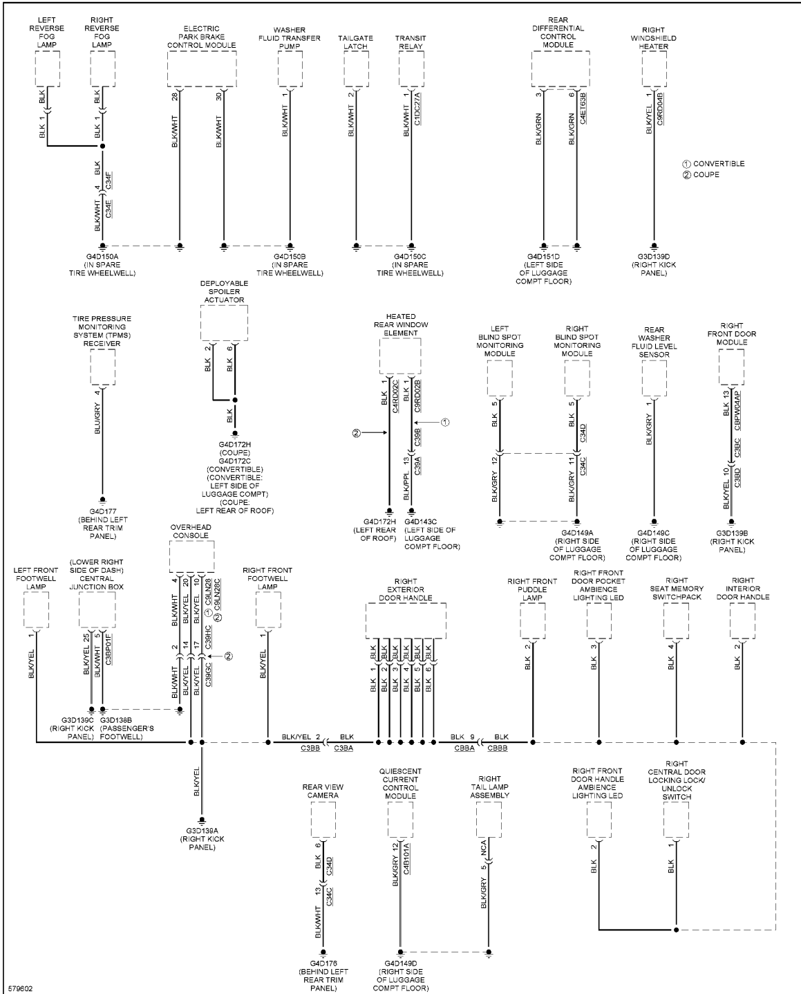
Fig. 49: Ground Distribution Circuit (6 of 6)
