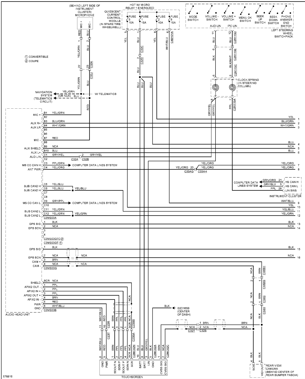
Fig. 111: Premium Radio Circuit, W/ Control Touch W/O Hi-line Audio (1 of 5)
