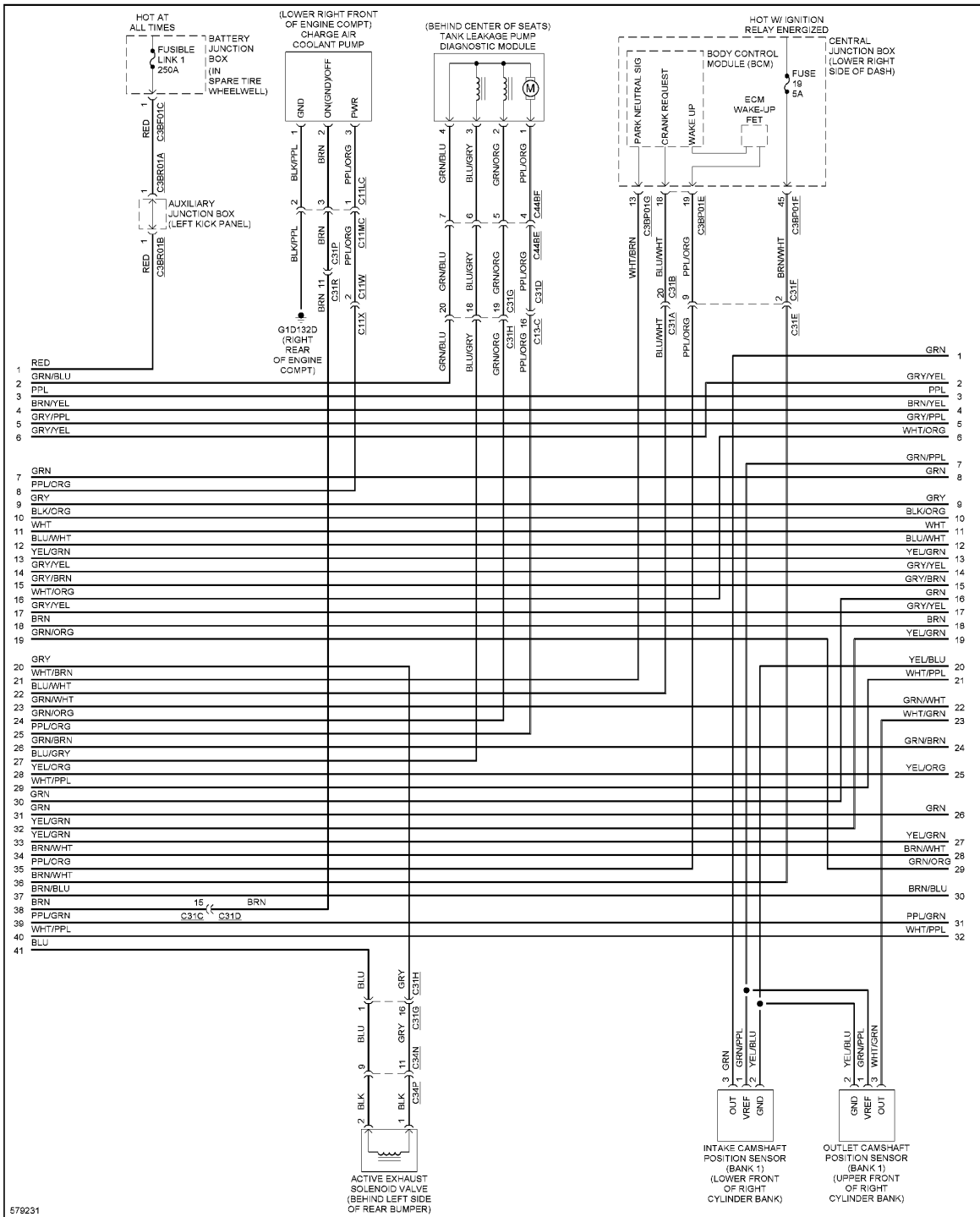
Fig. 25: 3.0L SC, Engine Performance Circuit (3 of 9)
