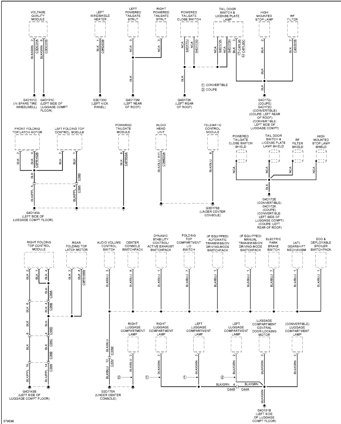
Fig. 46: Ground Distribution Circuit (3 of 6)
