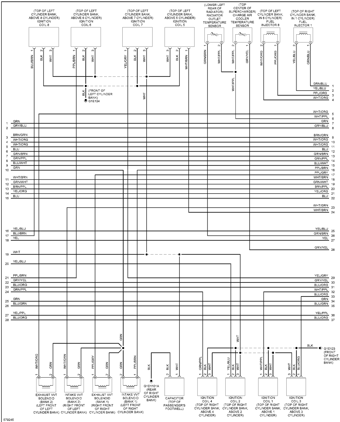
Fig. 39: 5.0L SC, Engine Performance Circuit (8 of 9)
