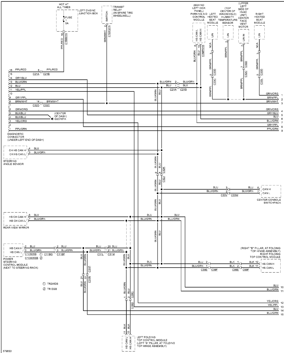
Fig. 9: Diagnostic Socket Circuit (1 of 4)
