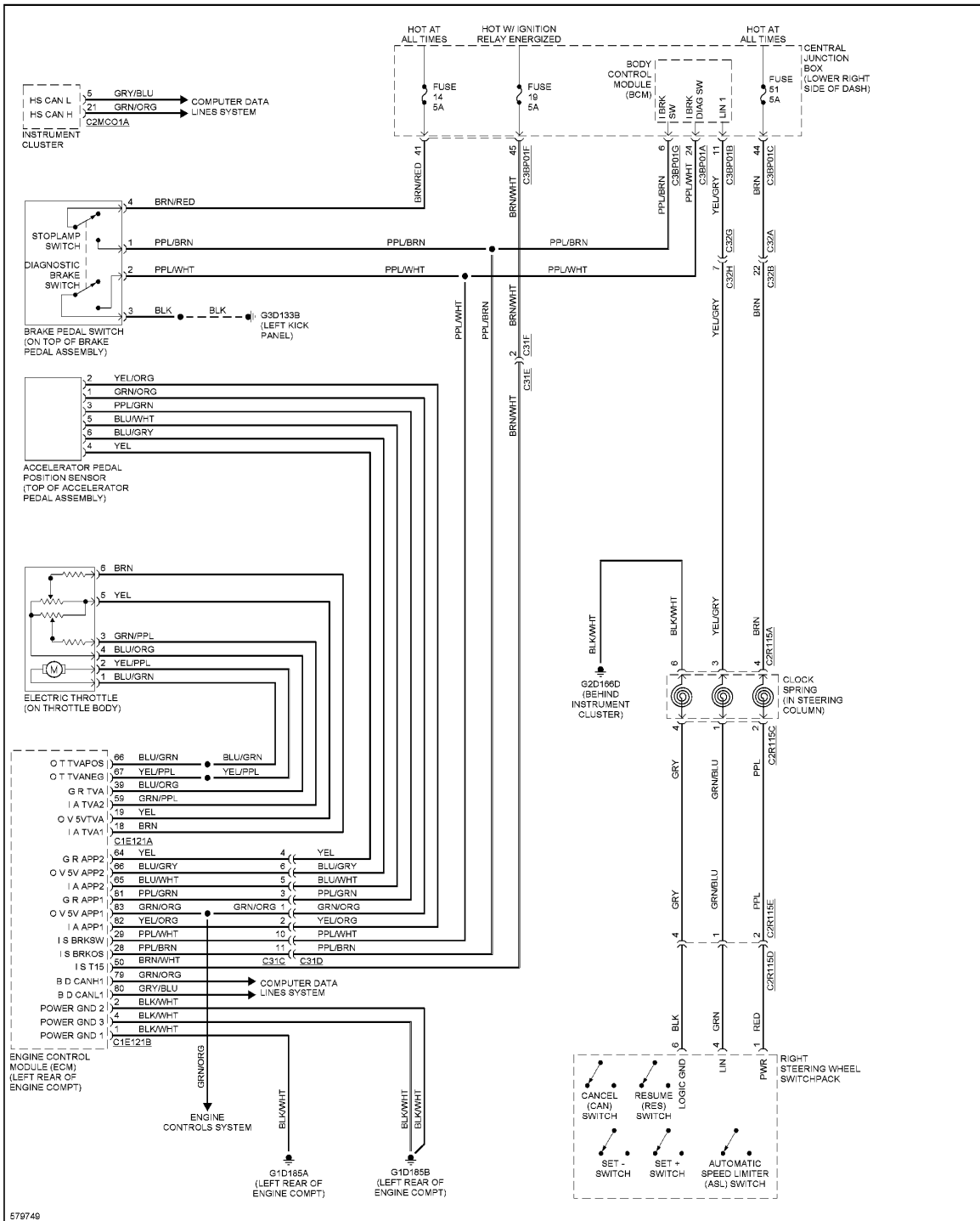
Fig. 16: Cruise Control Circuit
