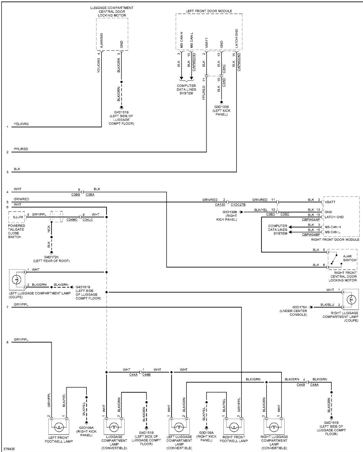
Fig. 56: Courtesy Lamps Circuit (2 of 2)
