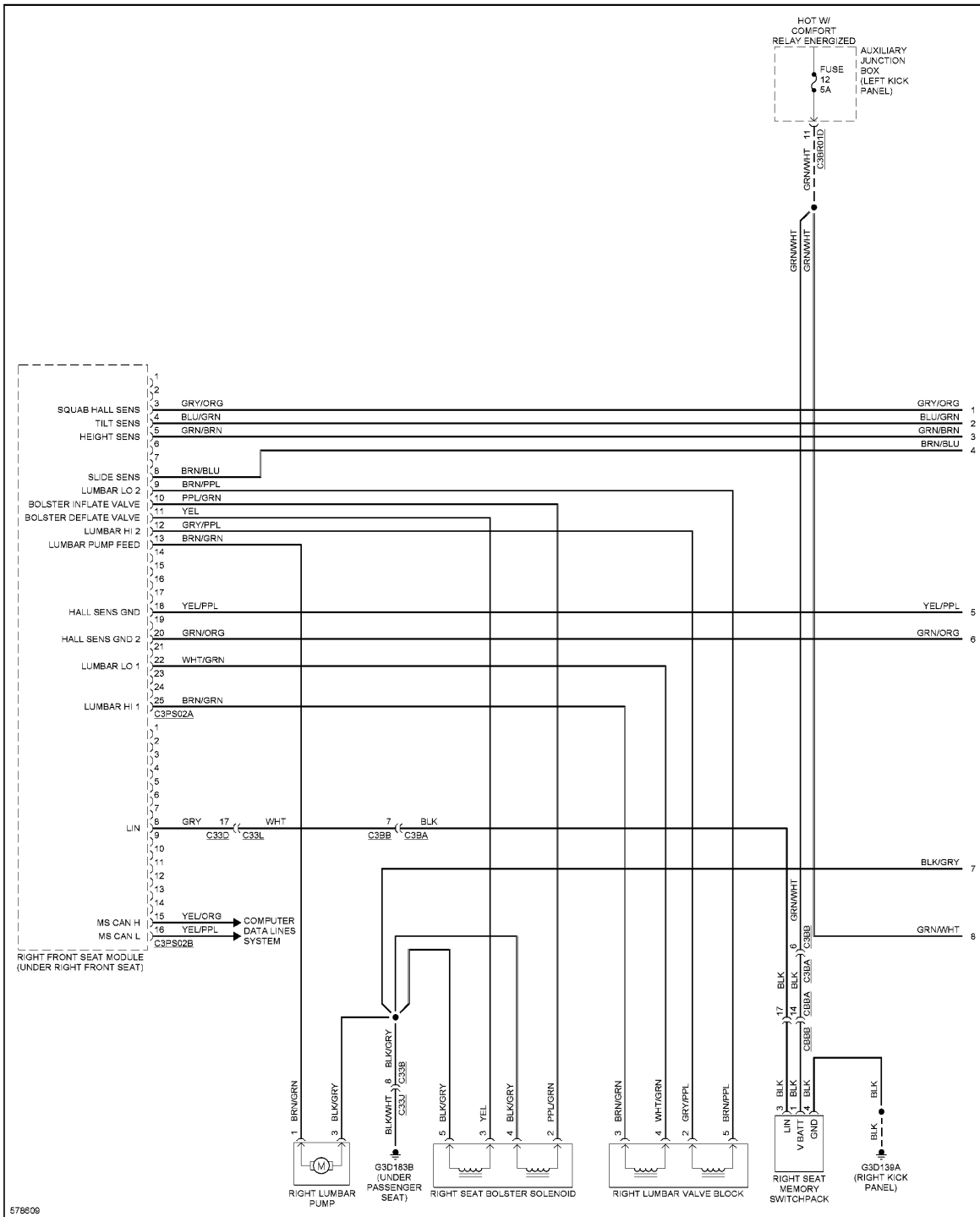
Fig. 64: Passenger's Memory Seat Circuit, 8-Way (1 of 2)
