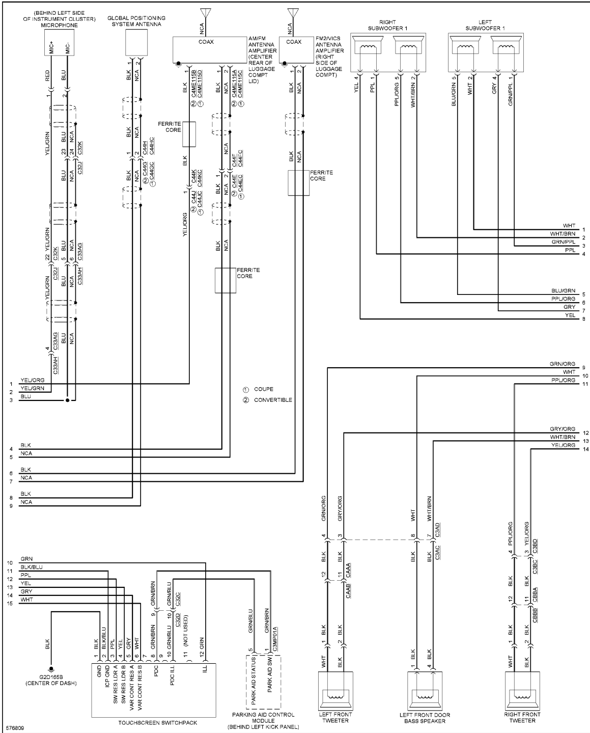
Fig. 120: Premium Radio Circuit, W/O Control Touch (5 of 6)
