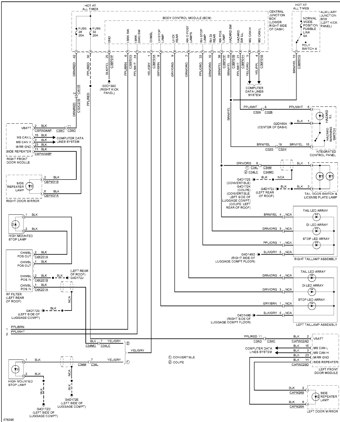
Fig. 43: Exterior Lamps Circuit (2 of 2)
