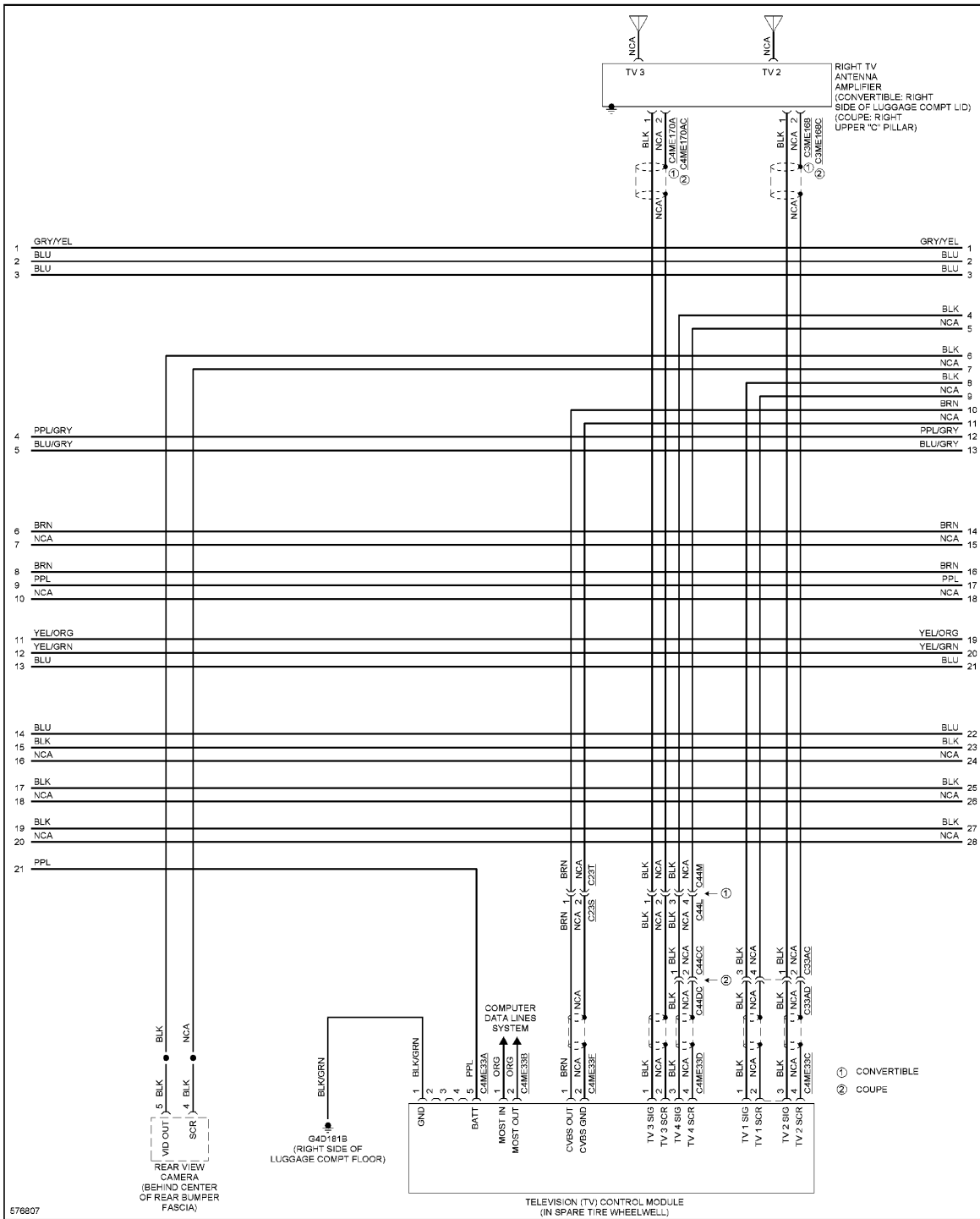
Fig. 118: Premium Radio Circuit, W/O Control Touch (3 of 6)
