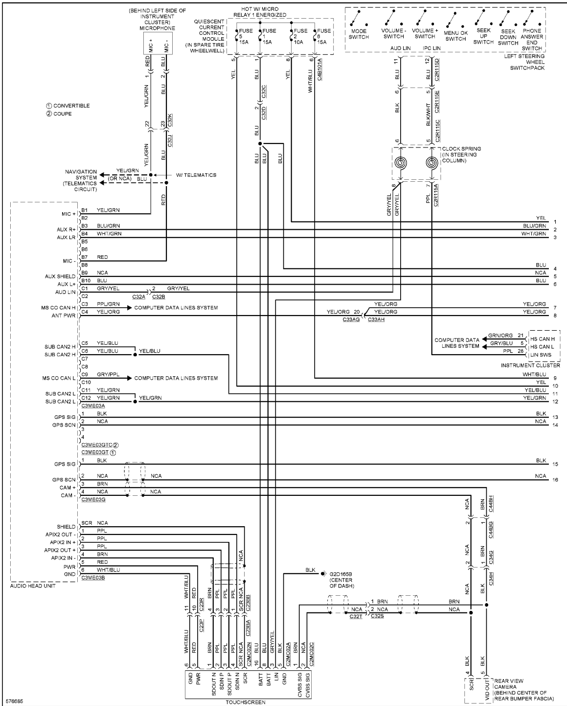
Fig. 73: Navigation Circuit, W/ Control Touch W/O Hi-line Audio (1 of 5)
