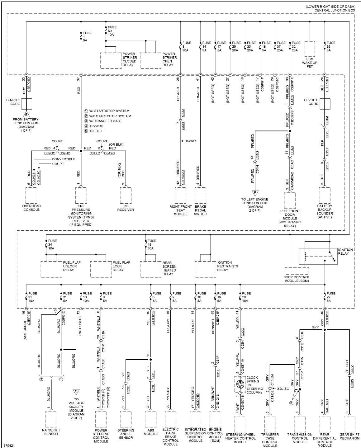
Fig. 90: Power Distribution Circuit (3 of 7)
