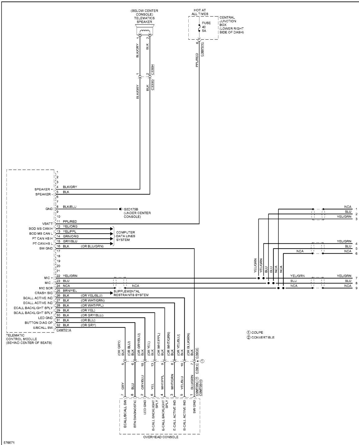
Fig. 86: Telematics Circuit (1 of 2)
