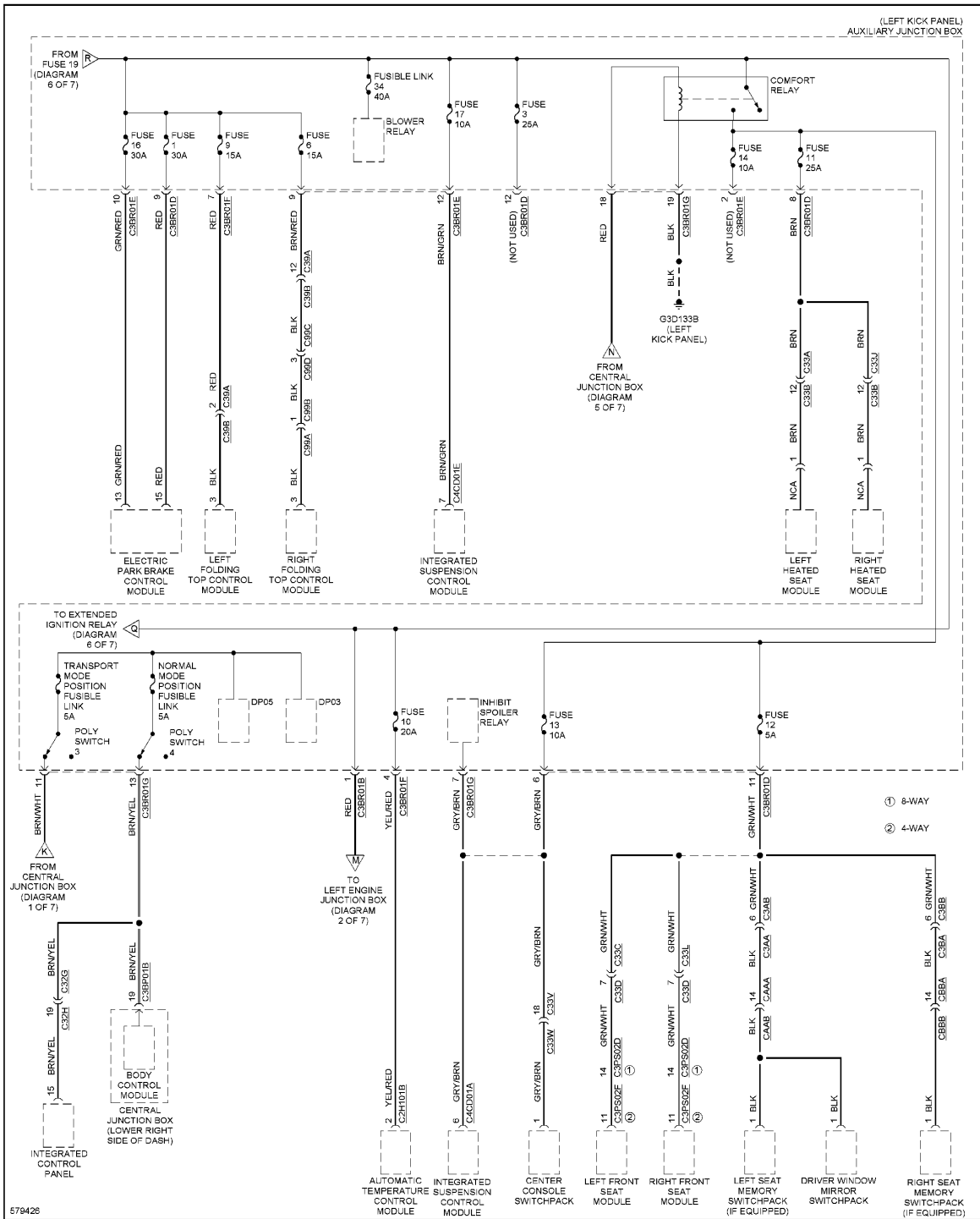
Fig. 94: Power Distribution Circuit (7 of 7)
