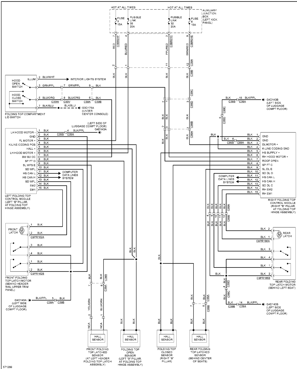
Fig. 103: Power Top/Sunroof Circuit
