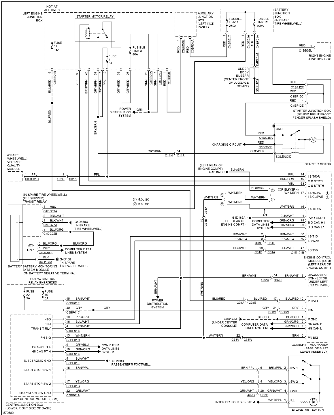
Fig. 126: Starting Circuit
