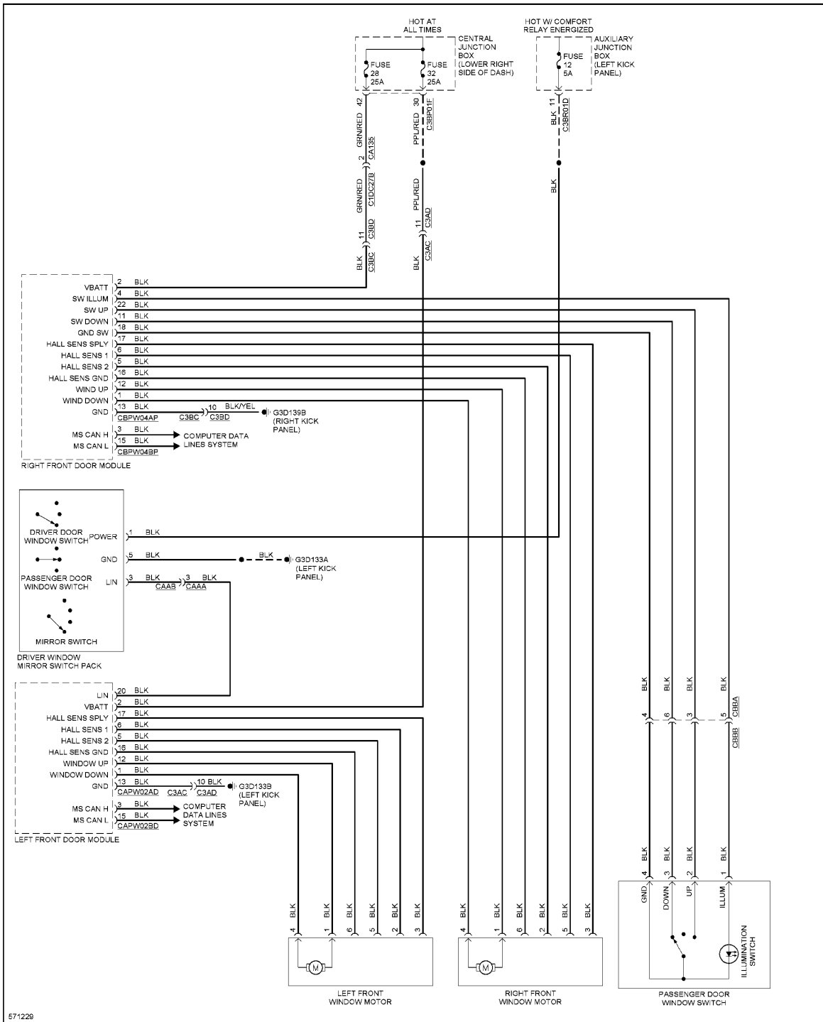
Fig. 104: Power Windows Circuit
