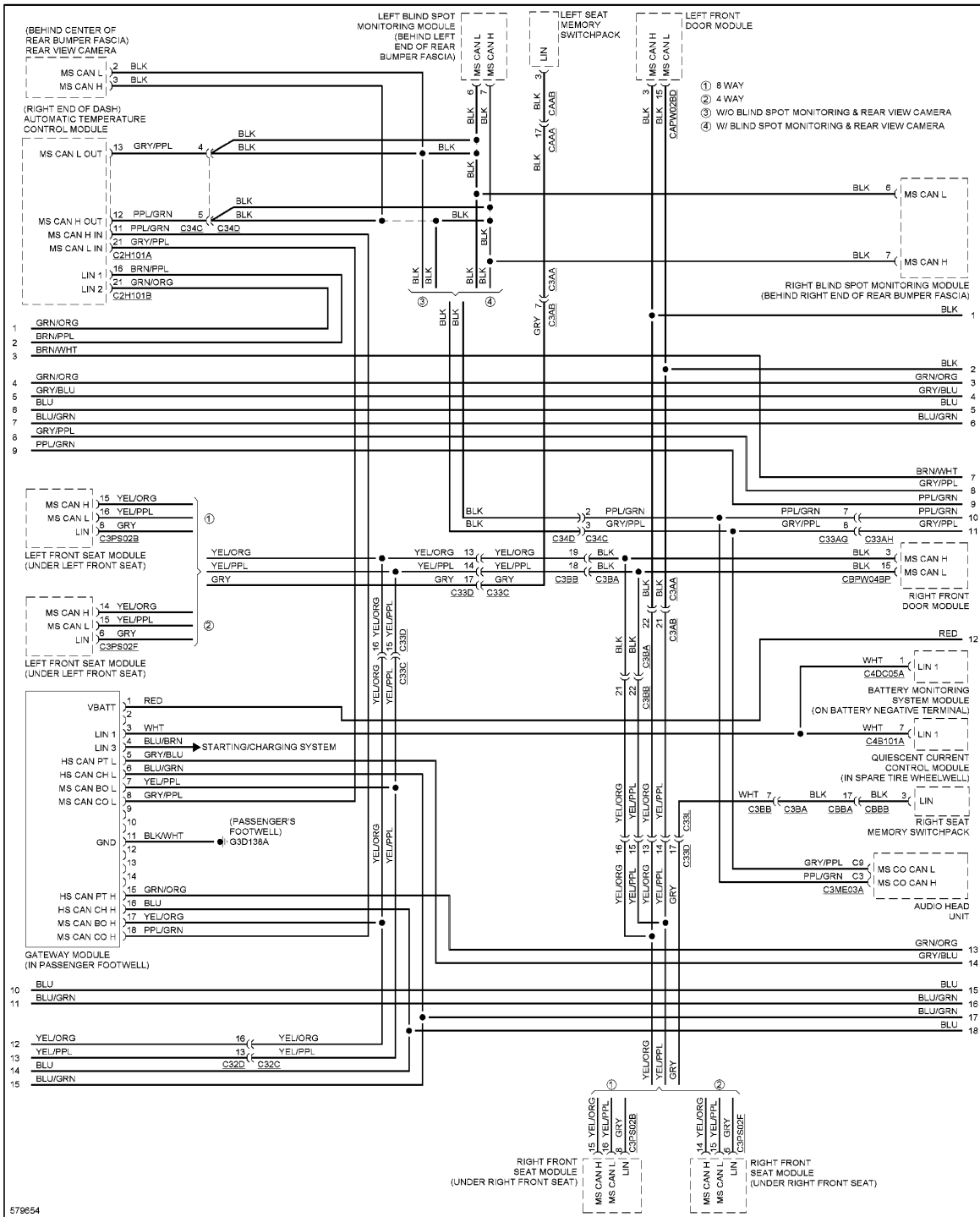
Fig. 10: Diagnostic Socket Circuit (2 of 4)
