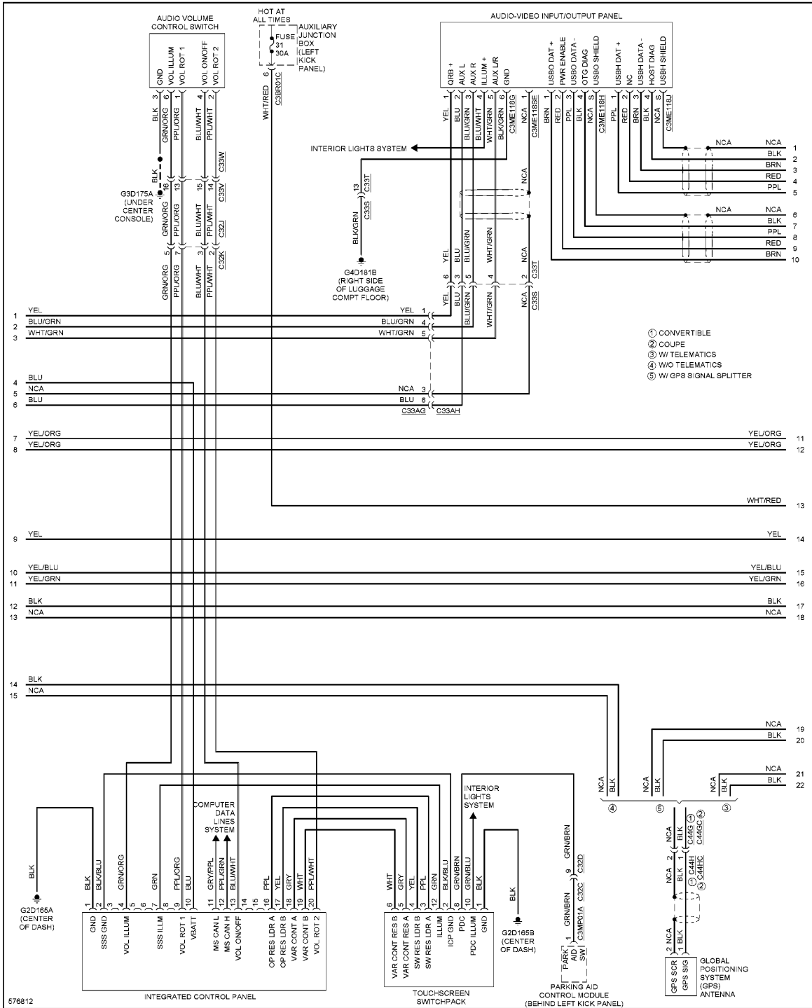
Fig. 107: Premium Radio Circuit, W/ Control Touch & Hi-line Audio (2 of 5)
