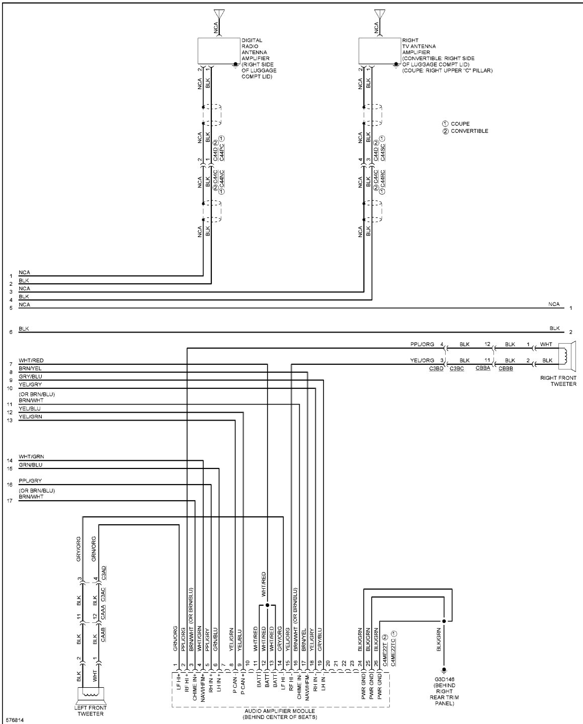
Fig. 109: Premium Radio Circuit, W/ Control Touch & Hi-line Audio (4 of 5)
