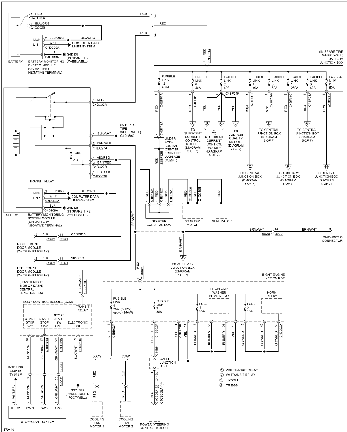
Fig. 88: Power Distribution Circuit (1 of 7)
