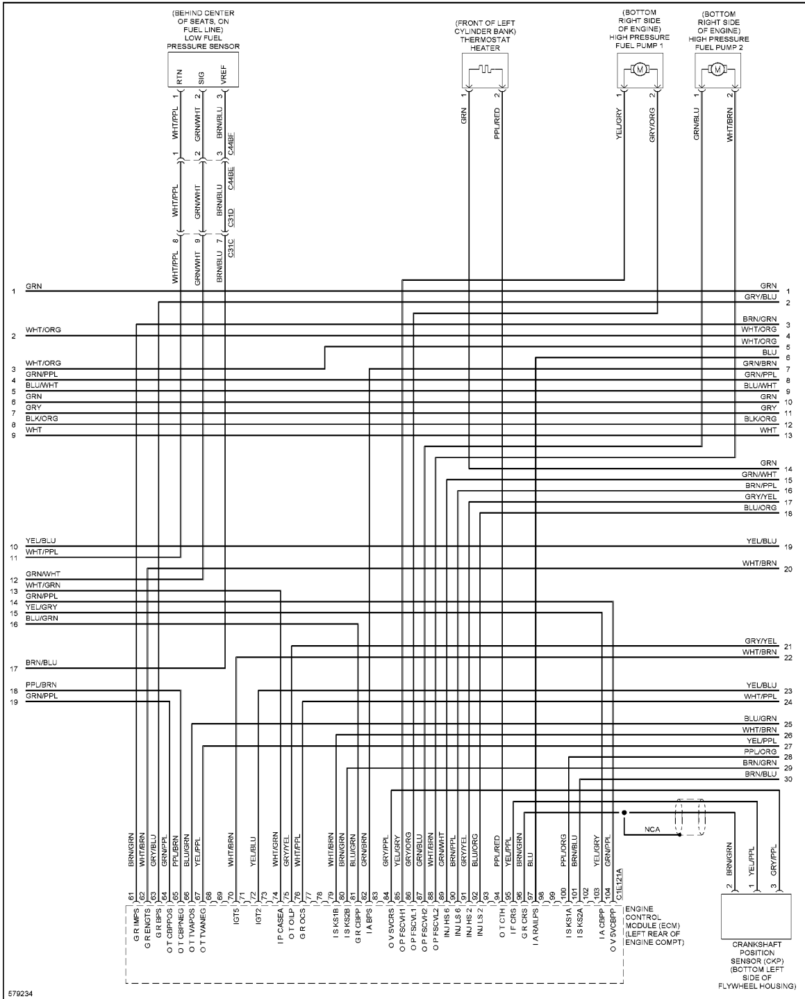
Fig. 28: 3.0L SC, Engine Performance Circuit (6 of 9)
