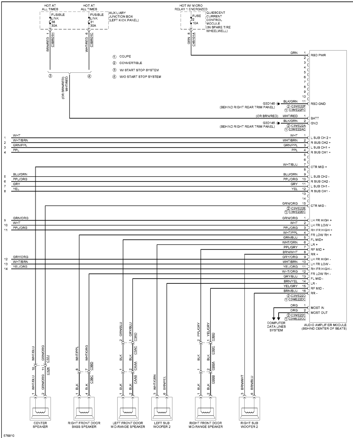
Fig. 121: Premium Radio Circuit, W/O Control Touch (6 of 6)
