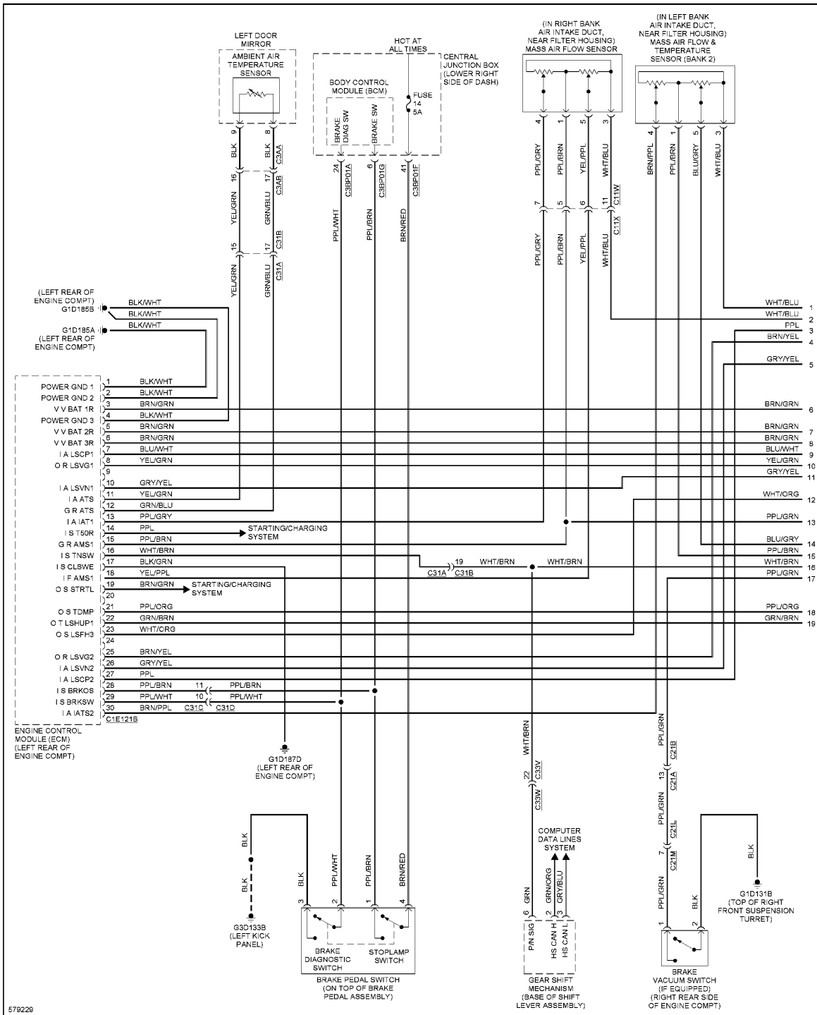
Fig. 23: 3.0L SC, Engine Performance Circuit (1 of 9)
