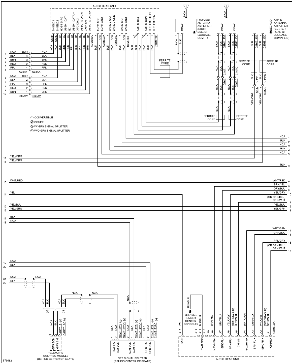
Fig. 70: Navigation Circuit, W/ Control Touch & Hi-line Audio (3 of 5)
