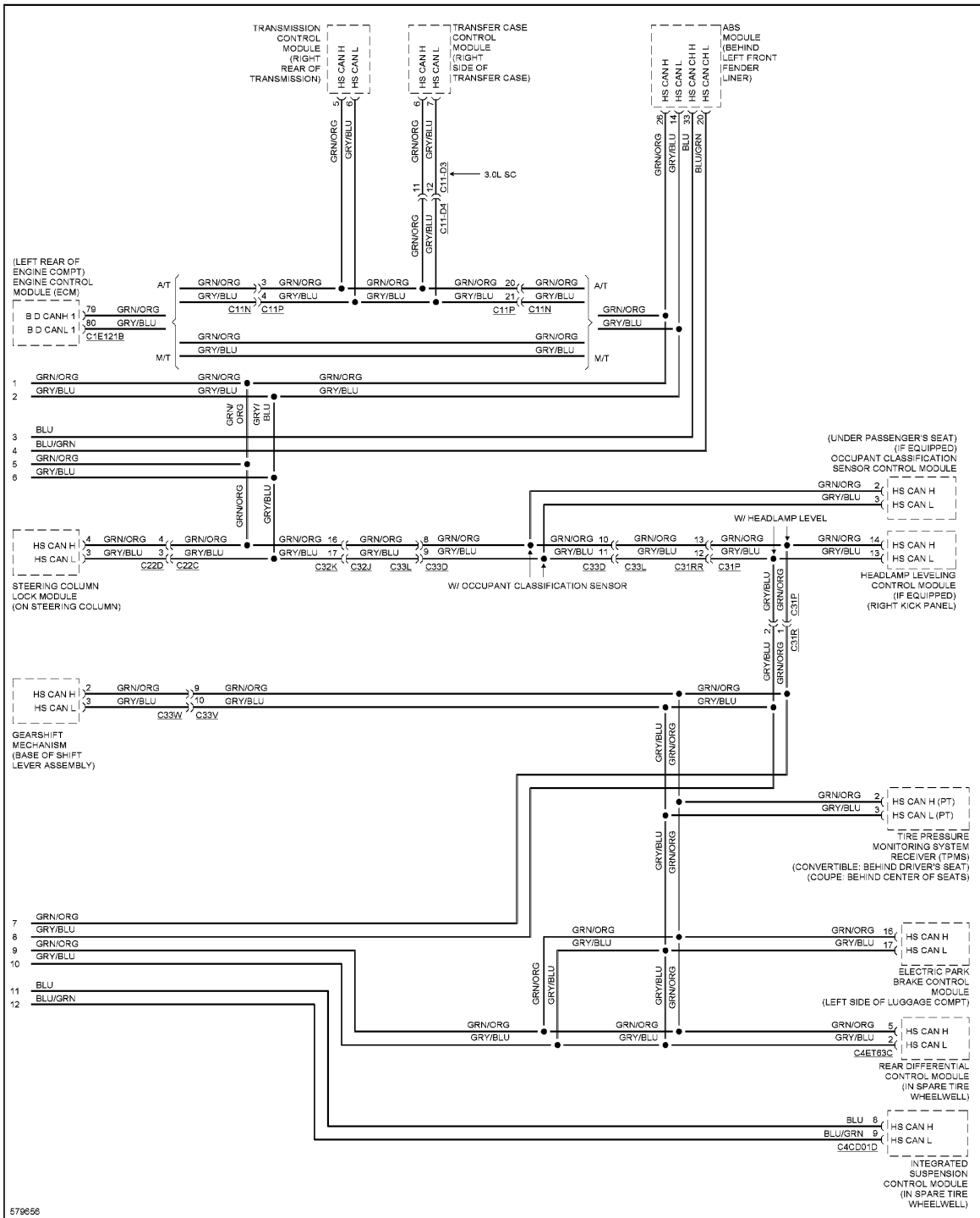
Fig. 12: Diagnostic Socket Circuit (4 of 4)
