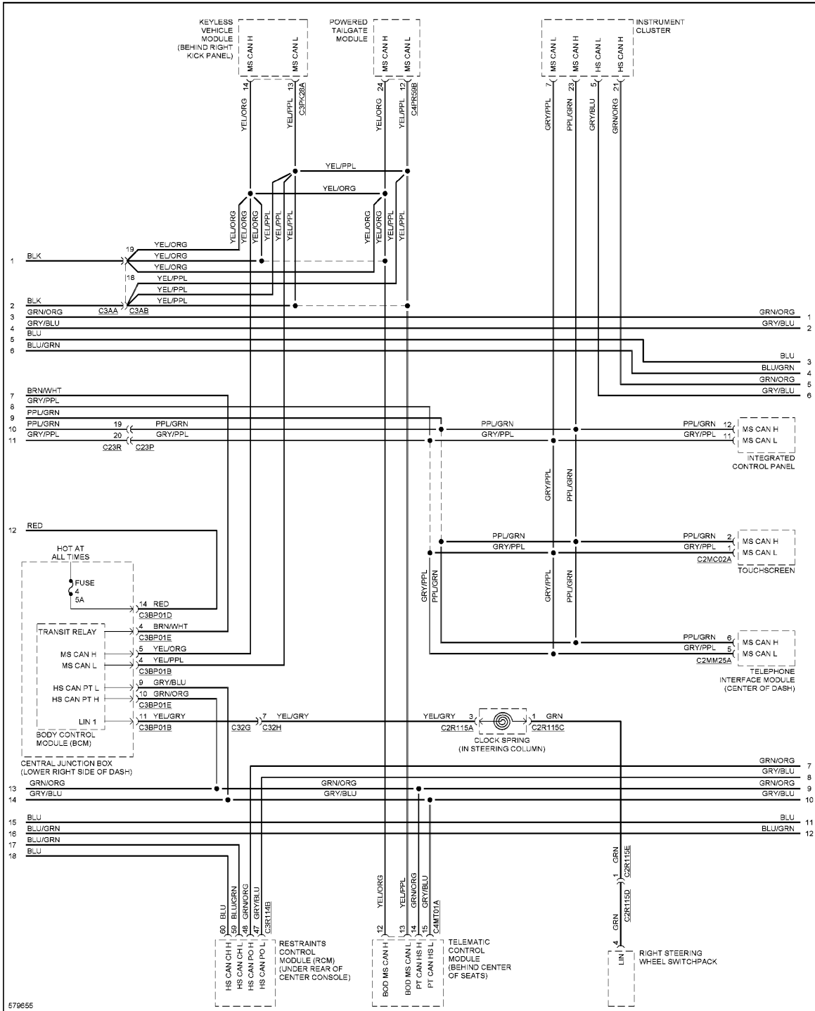
Fig. 11: Diagnostic Socket Circuit (3 of 4)
