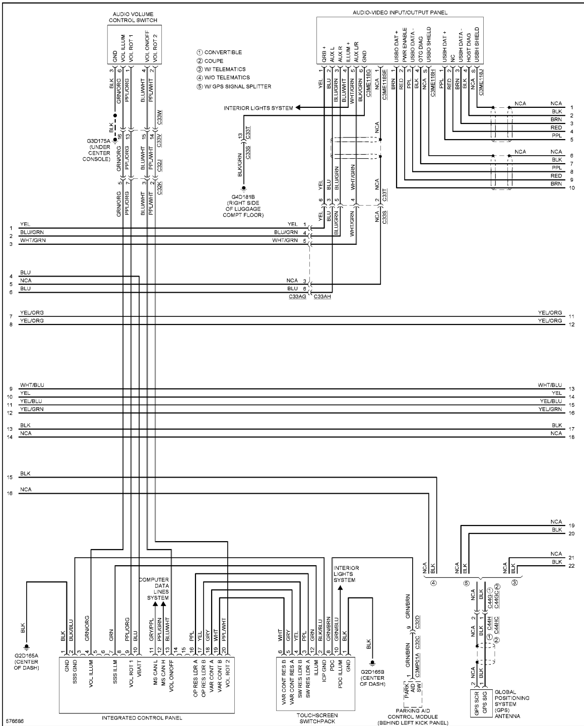
Fig. 74: Navigation Circuit, W/ Control Touch W/O Hi-line Audio (2 of 5)
