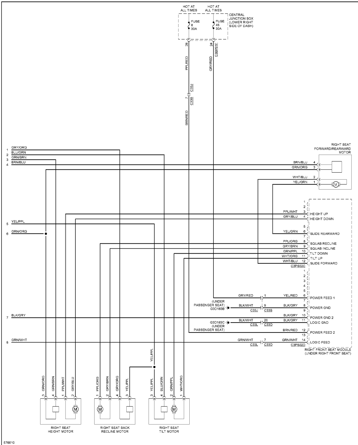
Fig. 65: Passenger's Memory Seat Circuit, 8-Way (2 of 2)
