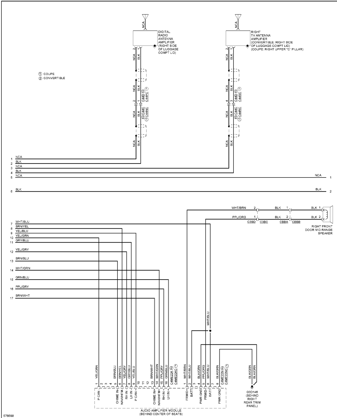
Fig. 76: Navigation Circuit, W/ Control Touch W/O Hi-line Audio (4 of 5)
