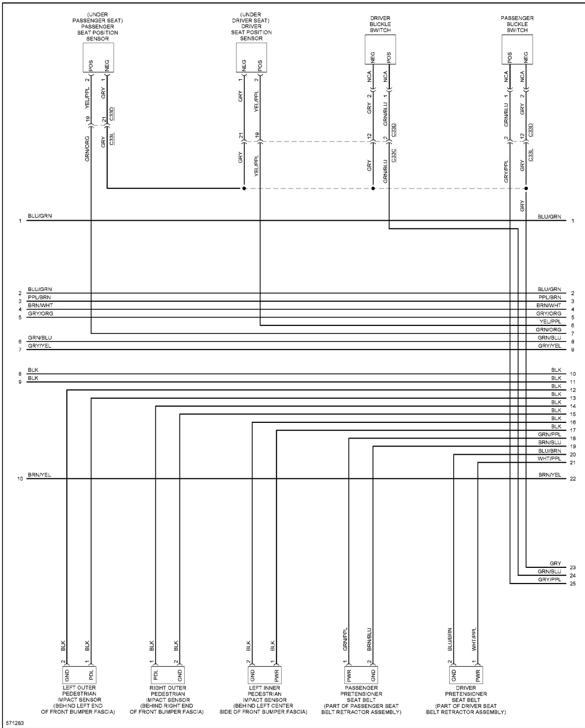
Fig. 129: Supplemental Restraints Circuit (3 of 4)
