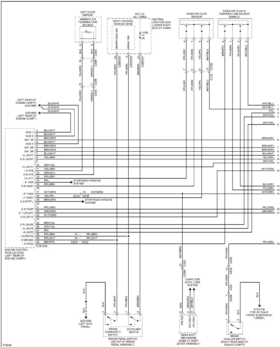
Fig. 32: 5.0L SC, Engine Performance Circuit (1 of 9)
