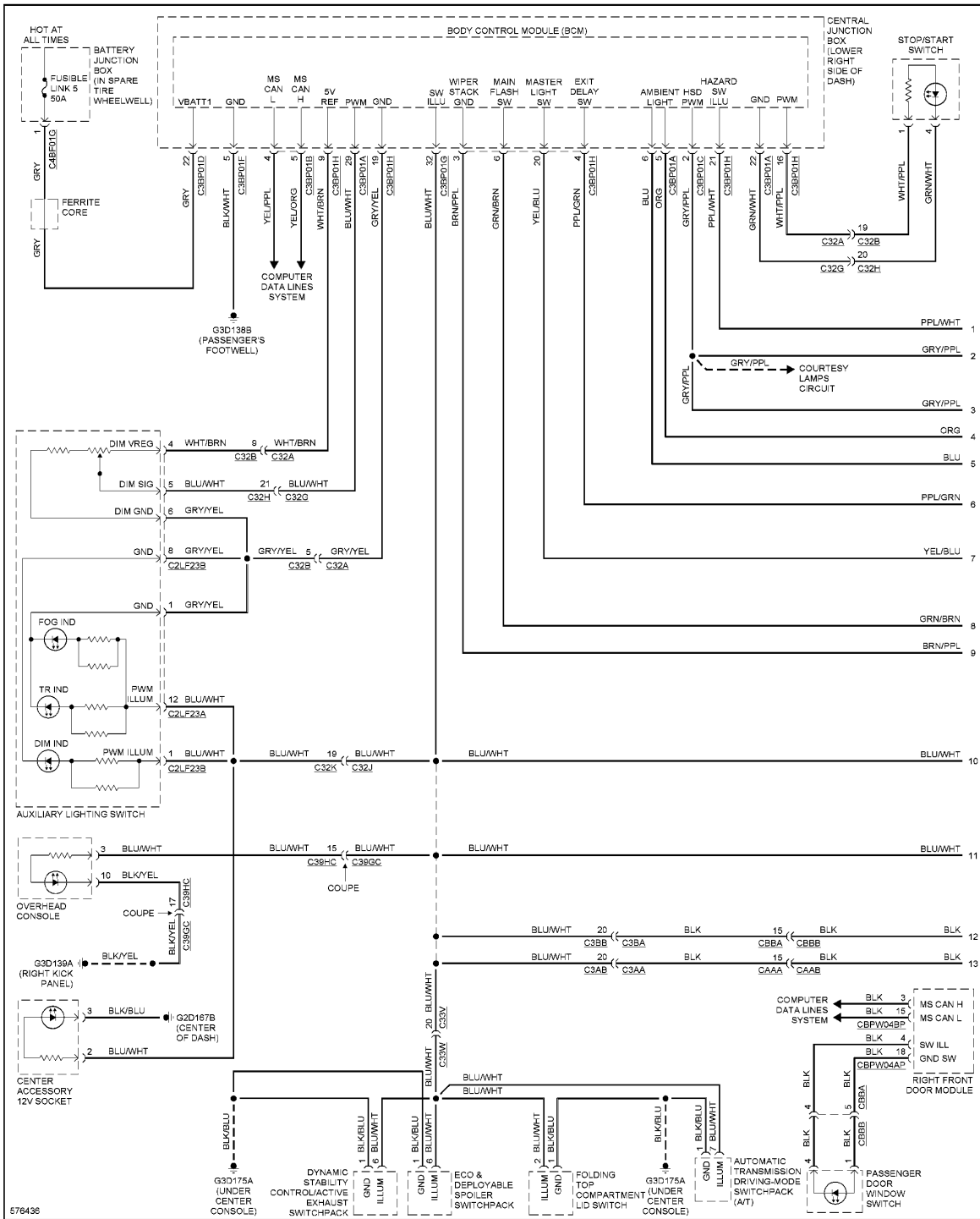
Fig. 57: Instrument Illumination Circuit (1 of 2)
