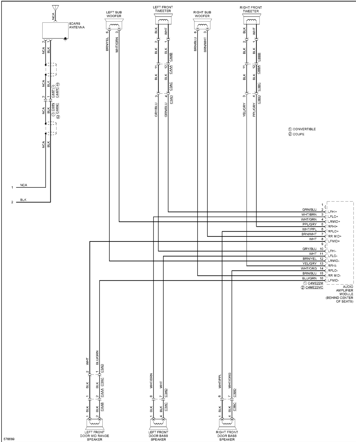
Fig. 77: Navigation Circuit, W/ Control Touch W/O Hi-line Audio (5 of 5)
