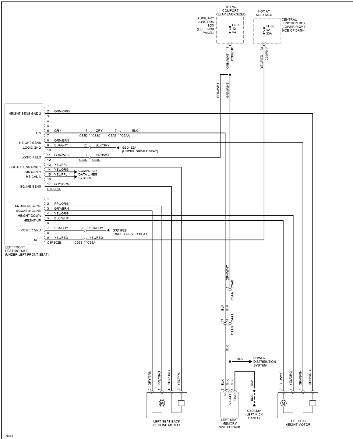
Fig. 59: Driver's Memory Seat Circuit, 4-Way
