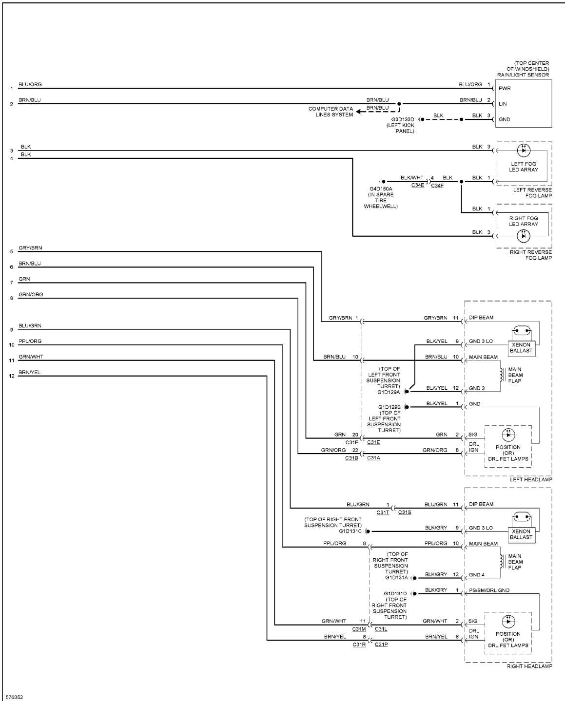
Fig. 52: Headlamps Circuit (2 of 2)
