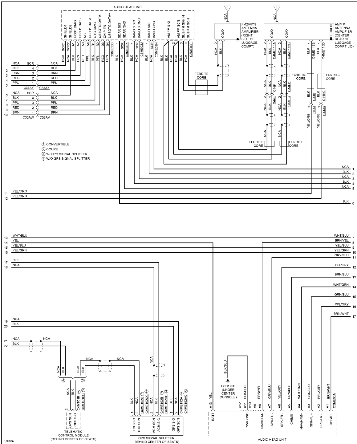
Fig. 75: Navigation Circuit, W/ Control Touch W/O Hi-line Audio (3 of 5)
