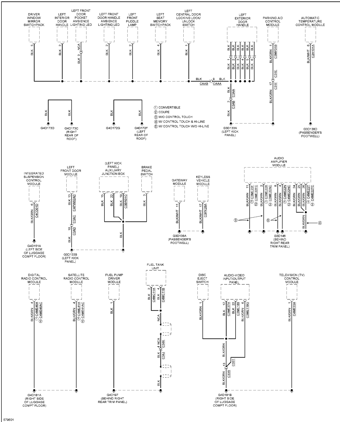
Fig. 48: Ground Distribution Circuit (5 of 6)
