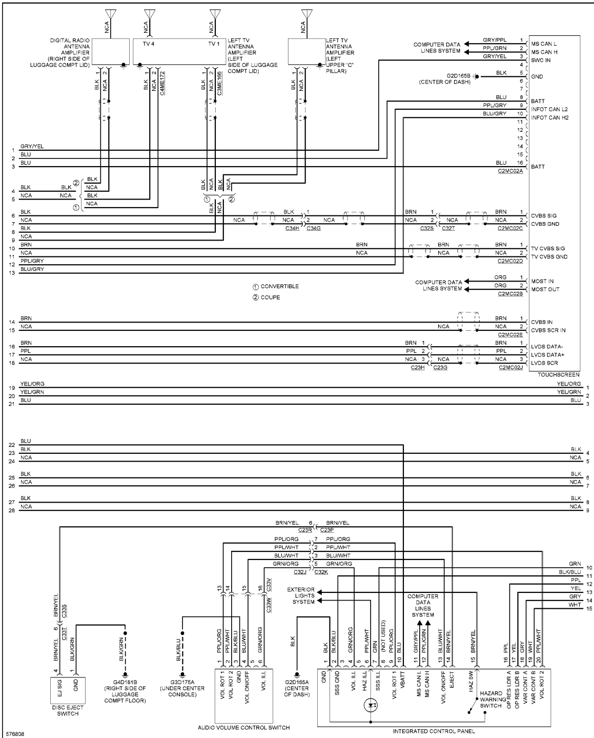
Fig. 119: Premium Radio Circuit, W/O Control Touch (4 of 6)
