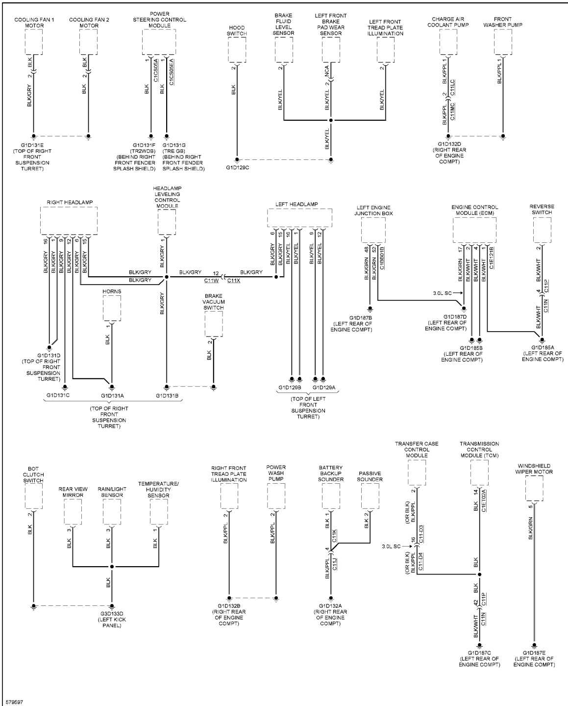
Fig. 44: Ground Distribution Circuit (1 of 6)
