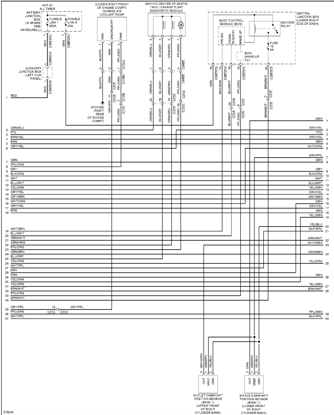
Fig. 34: 5.0L SC, Engine Performance Circuit (3 of 9)
