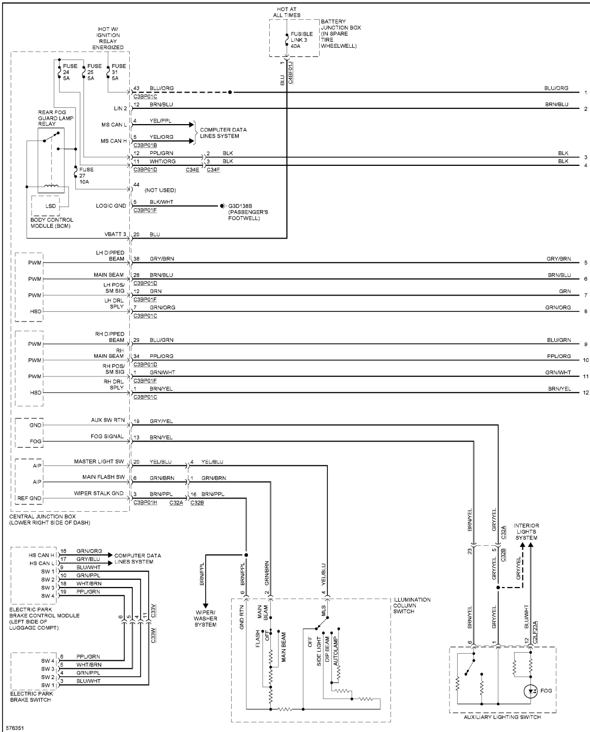
Fig. 51: Headlamps Circuit (1 of 2)
