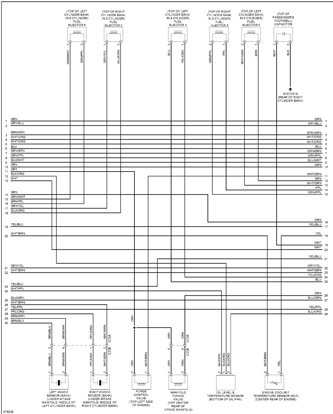
Fig. 29: 3.0L SC, Engine Performance Circuit (7 of 9)
