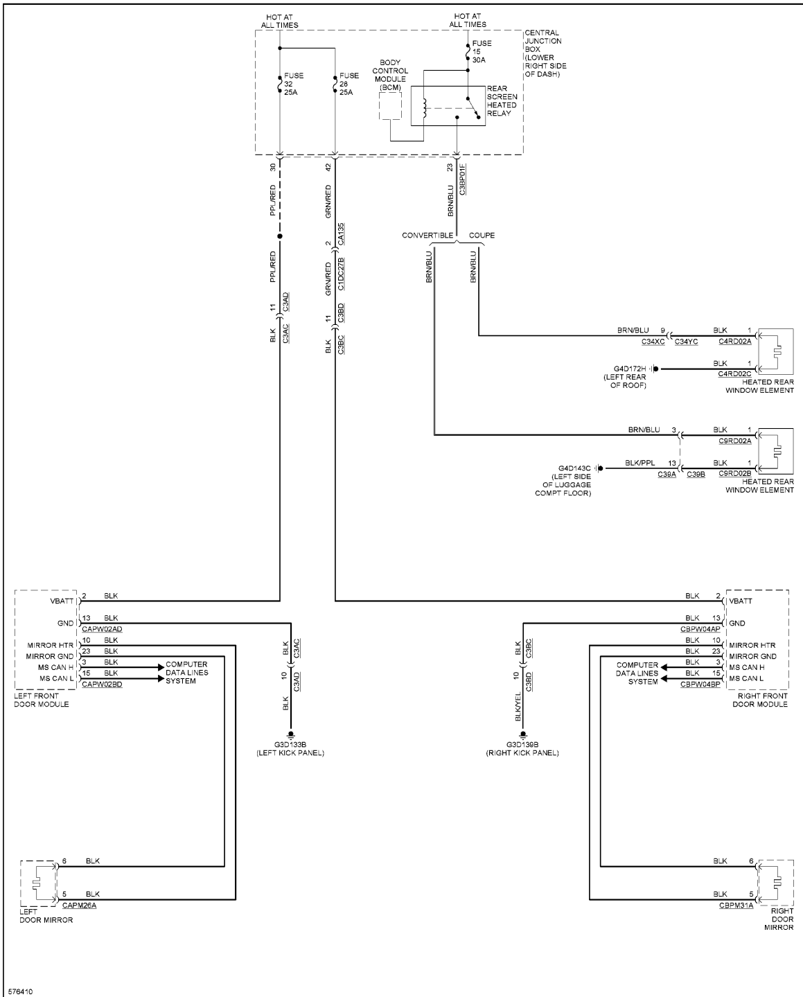
Fig. 18: Rear Defogger & Heated Mirrors Circuit
