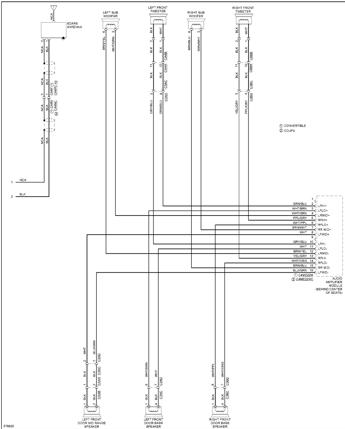
Fig. 115: Premium Radio Circuit, W/ Control Touch W/O Hi-line Audio (5 of 5)
