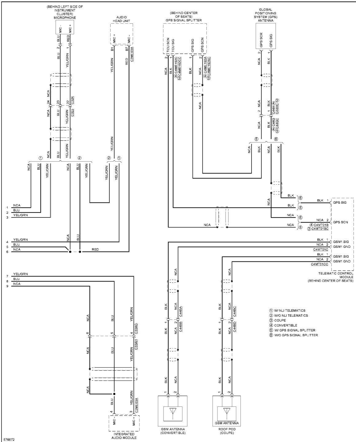
Fig. 87: Telematics Circuit (2 of 2)
