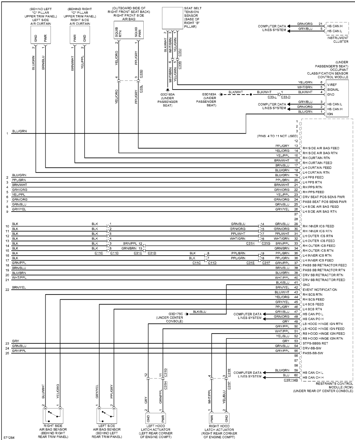
Fig. 130: Supplemental Restraints Circuit (4 of 4)
