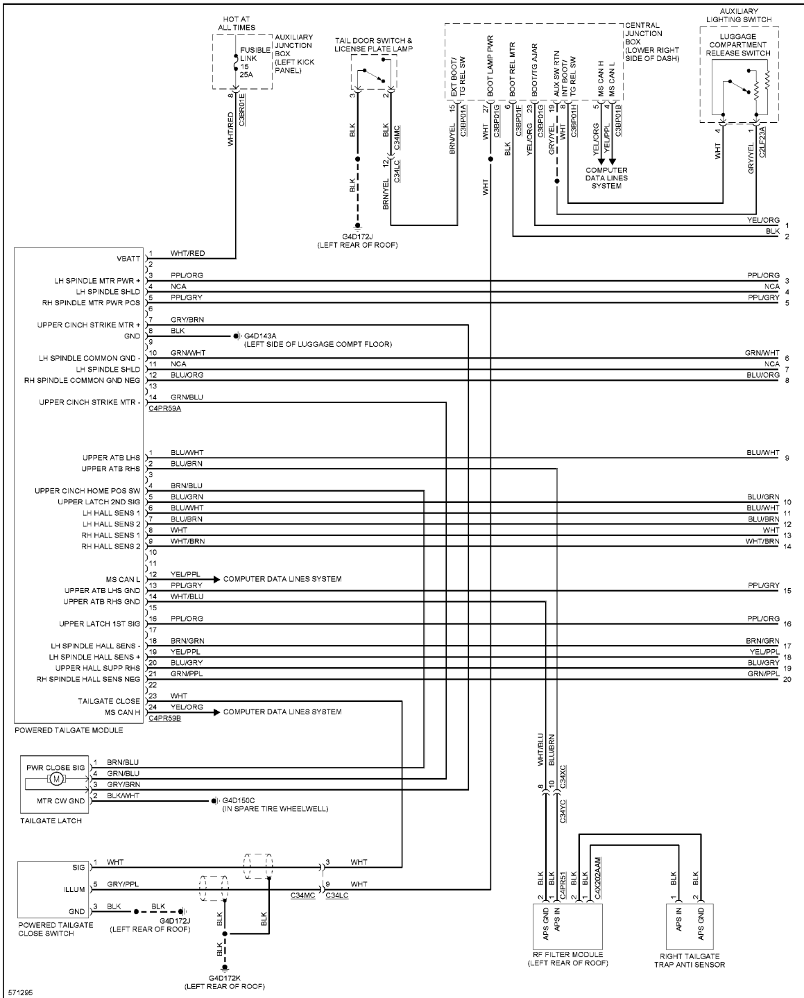
Fig. 133: Power Tailgate Circuit (1 of 2)
