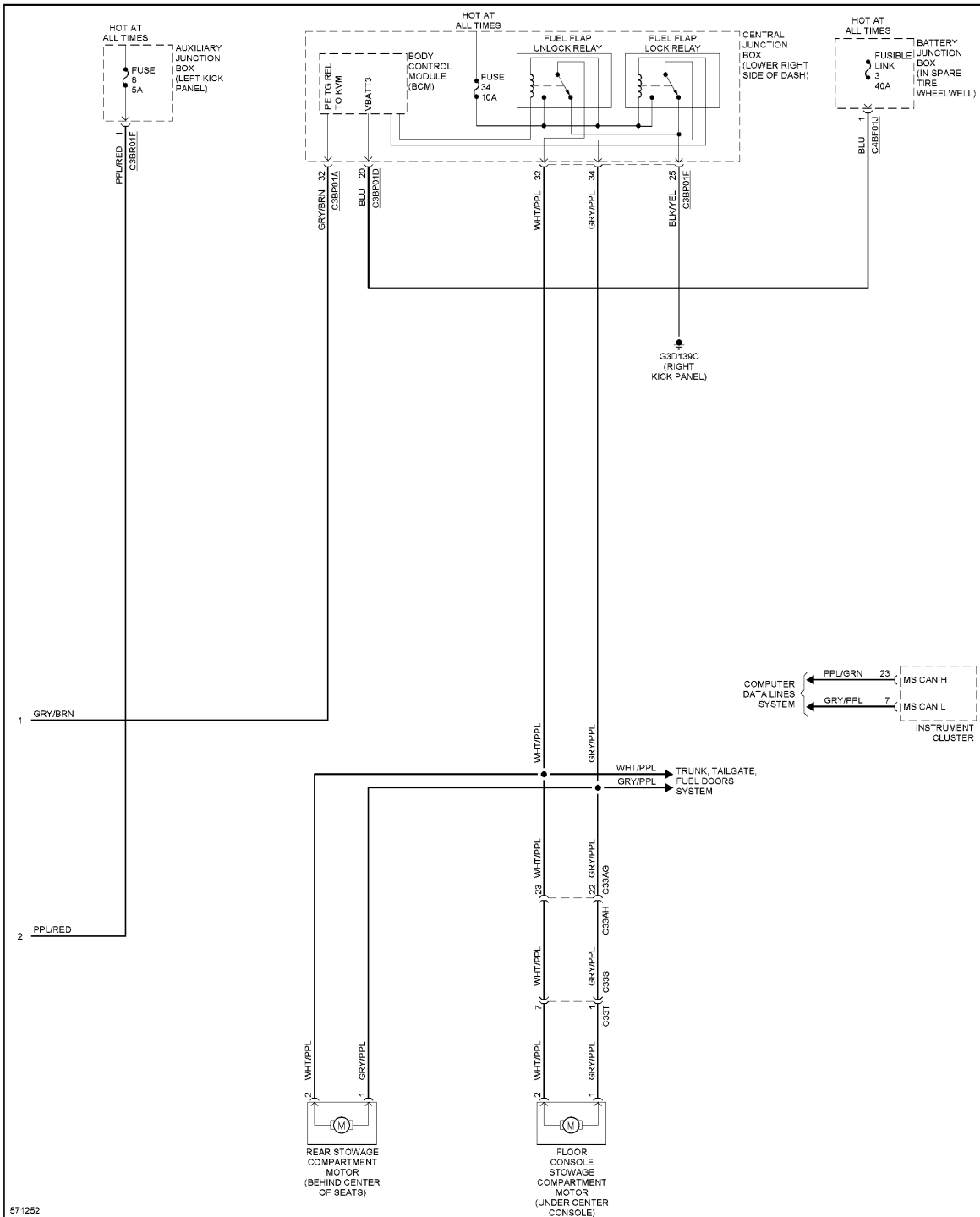
Fig. 98: Power Door Locks Circuit (4 of 4)
