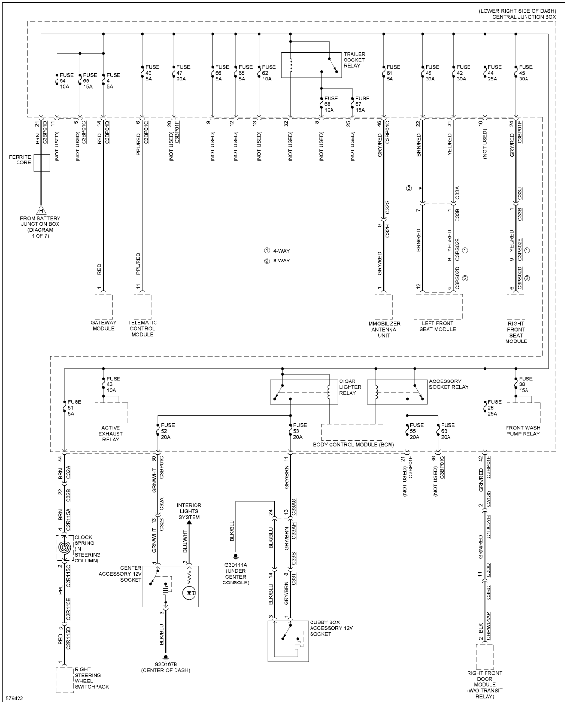
Fig. 91: Power Distribution Circuit (4 of 7)
