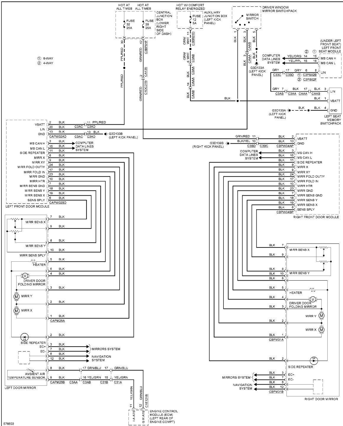
Fig. 62: Memory Mirrors Circuit
