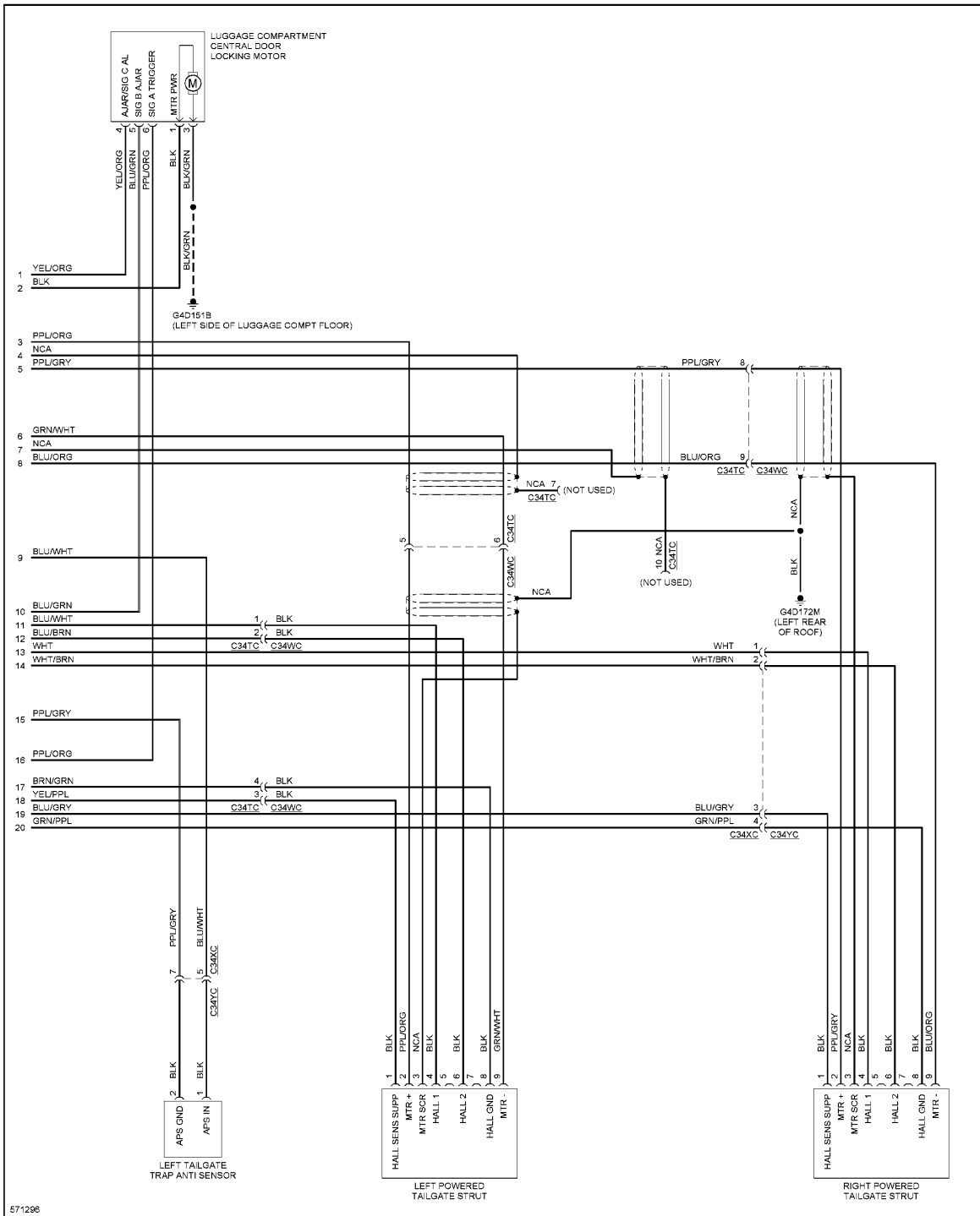
Fig. 134: Power Tailgate Circuit (2 of 2)
