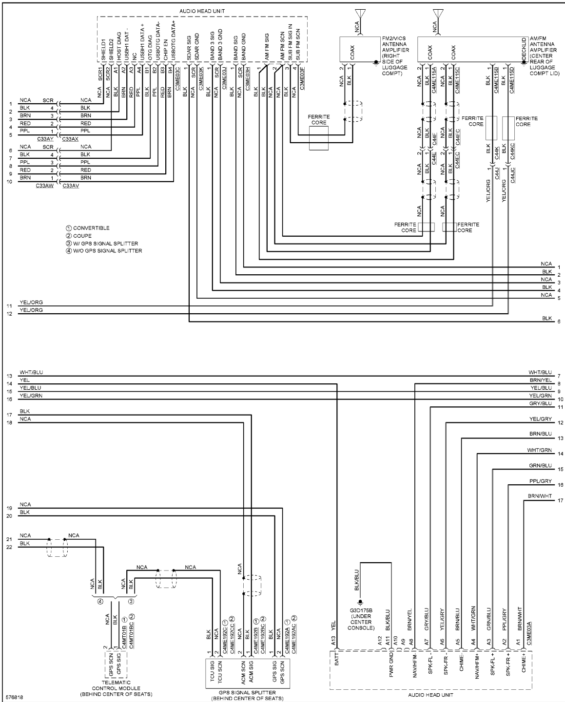
Fig. 113: Premium Radio Circuit, W/ Control Touch W/O Hi-line Audio (3 of 5)
