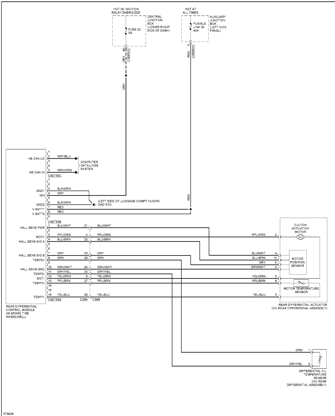
Fig. 132: Rear Differential Lock Circuit
