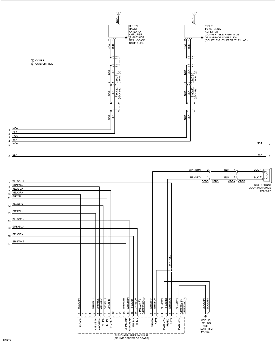
Fig. 114: Premium Radio Circuit, W/ Control Touch W/O Hi-line Audio (4 of 5)
