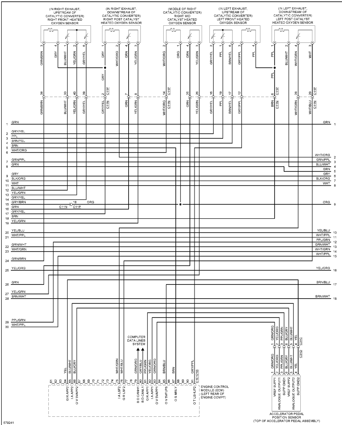
Fig. 35: 5.0L SC, Engine Performance Circuit (4 of 9)
