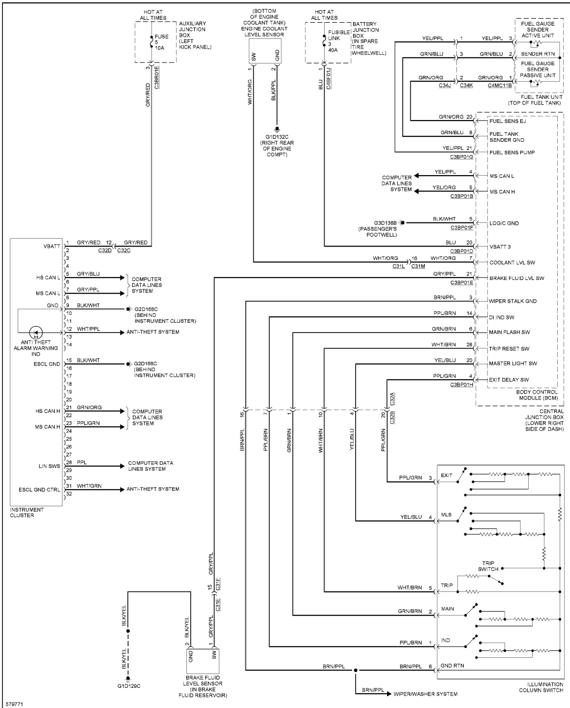
Fig. 54: Instrument Cluster Circuit
