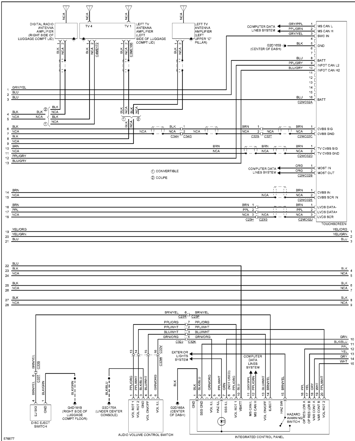
Fig. 81: Navigation Circuit, W/O Control Touch (4 of 6)
