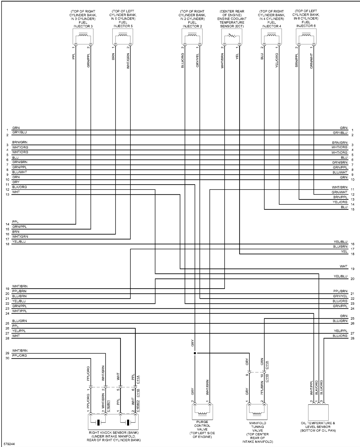
Fig. 38: 5.0L SC, Engine Performance Circuit (7 of 9)
