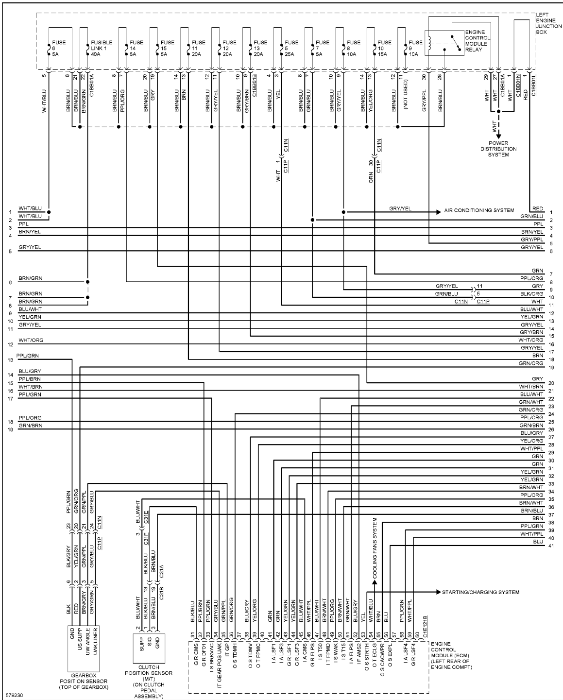
Fig. 24: 3.0L SC, Engine Performance Circuit (2 of 9)
