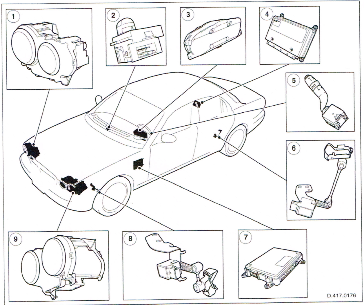
Fig. 106 Headlamp features
