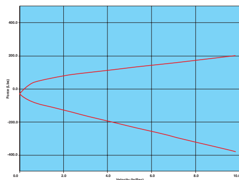
This graph depicts the Bilstein U37T linear piston combined with 37.4 mm cover plates. The result is valving with more "low-speed" control.
