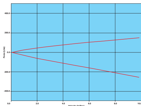
This graph was generated by a Bilstein U37T linear piston using 36.4 mm diameter cover plates resulting in a high bleed (or high frequency) style, short track linear valving.
