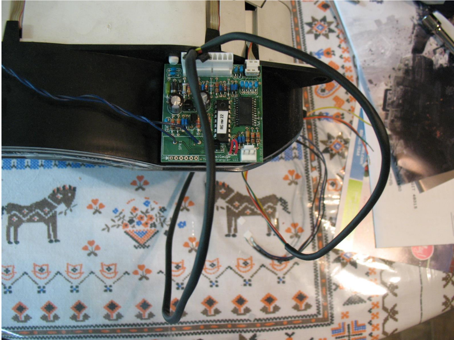
10 way Connector installed on the new Circuit Board
