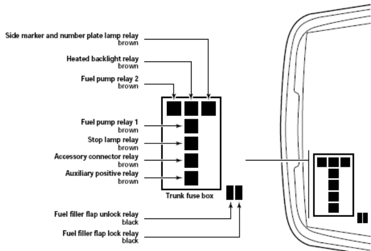
TRUNK RELAYS AND FUSE BOX
