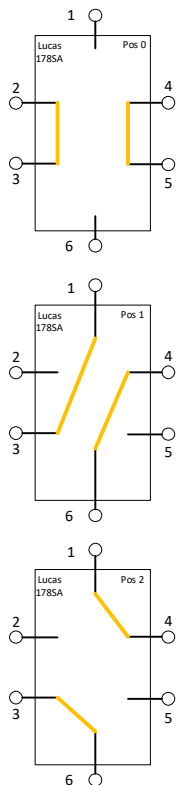
Circuit diagram
