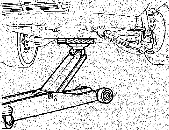
Front end (both wheels) jacking point
