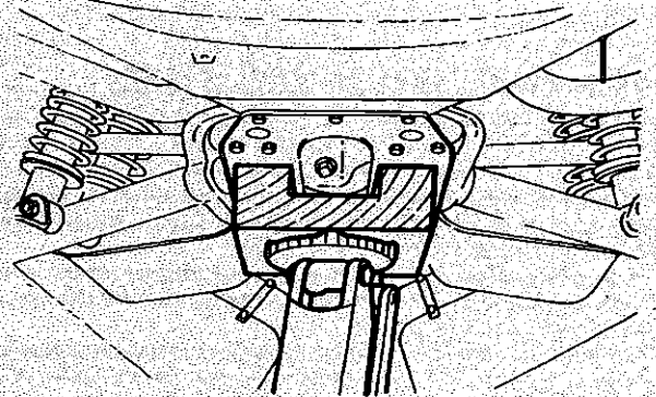
Rear end (both wheels) jacking point - note shaped block of wood
