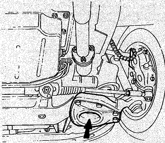
Front wheel jacking point
