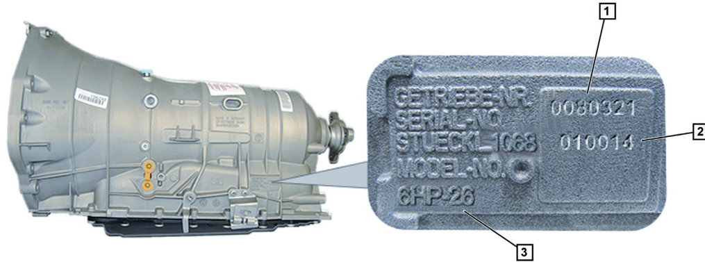
Fig. 1: 1 Serial Number, 2 Main Parts List, 3 Transmission Type
